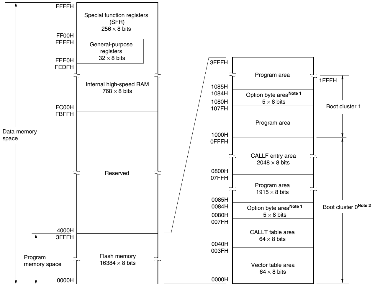
Figure 3-2. Memory Map ( \mu PD78F0501A, 78F0511A, 78F0521A, 78F0531A)
