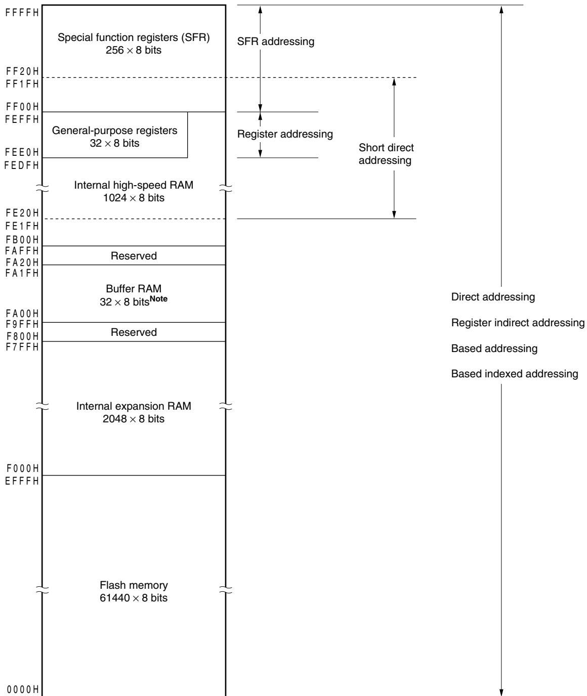
Figure 3-17. Correspondence Between Data Memory and Addressing (μPD78F0515A, 78F0525A, 78F0535A, 78F0545A, 78F0515DA)
