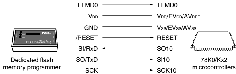
Figure 27-4. Communication with Dedicated Flash memory programmer (CSI10)
