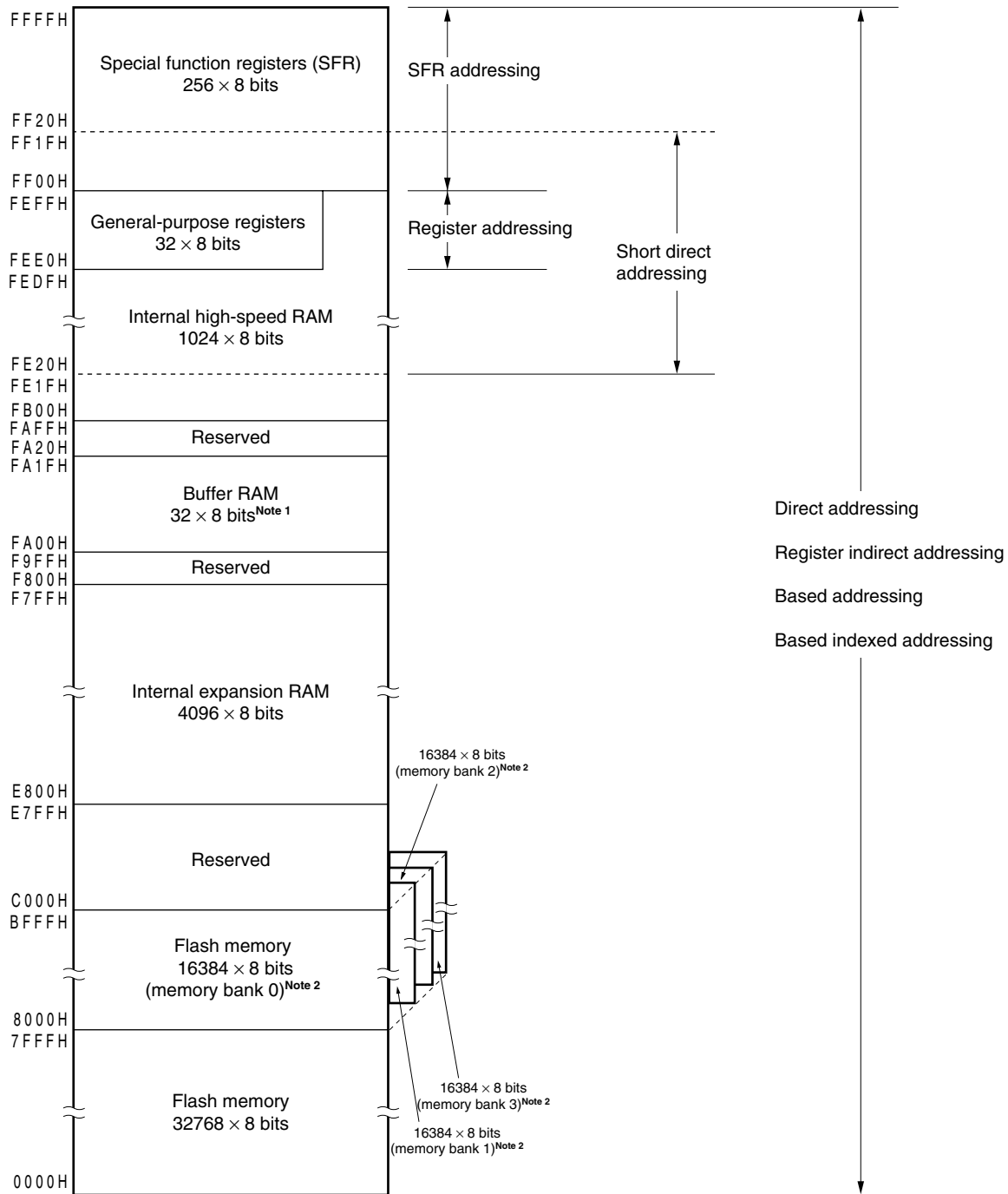
Figure 3-18. Correspondence Between Data Memory and Addressing ( \mu PD78F0526A, 78F0536A, 78F0546A)
