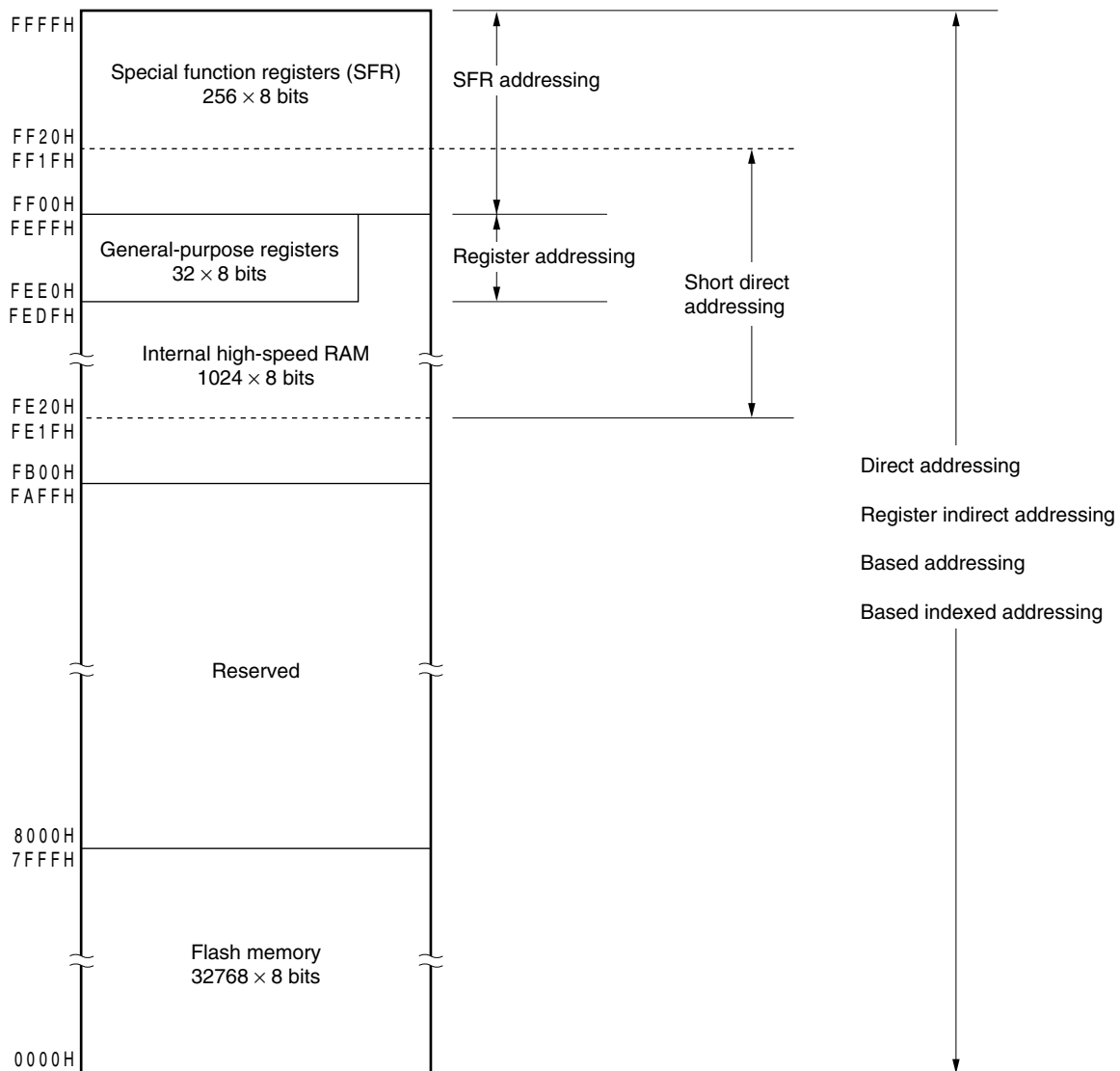
Figure 3-15. Correspondence Between Data Memory and Addressing ( \mu PD78F0503A, 78F0513A, 78F0523A, 78F0533A, 78F0503DA, and 78F0513DA)
