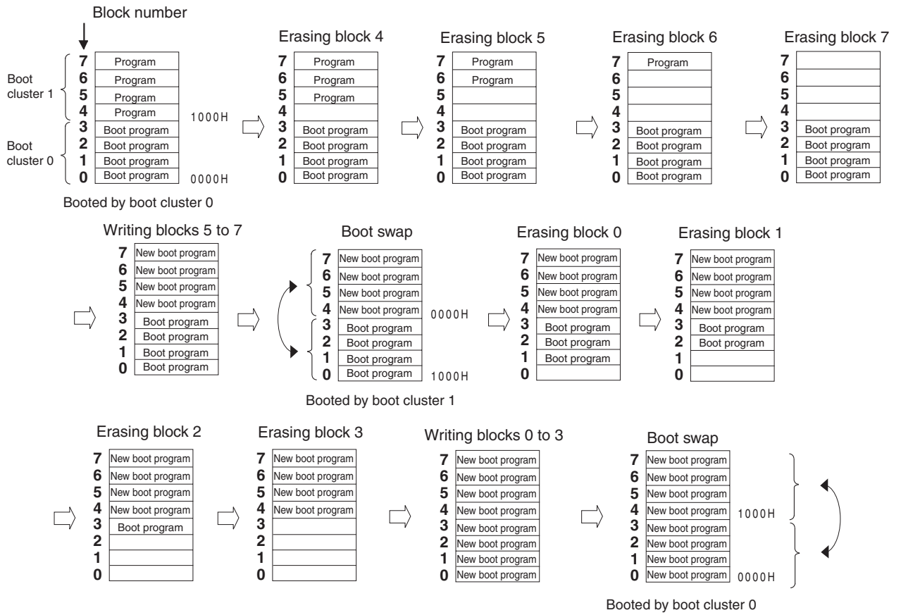
Figure 27-16. Example of Executing Boot Swapping
