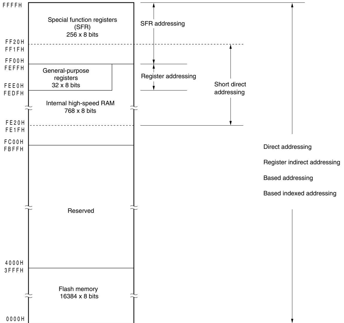
Figure 3-13. Correspondence Between Data Memory and Addressing (μPD78F0501A, 78F0511A, 78F0521A, and 78F0531A)
