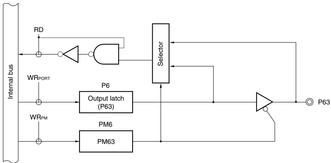
Figure 5-19. Block Diagram of P63
