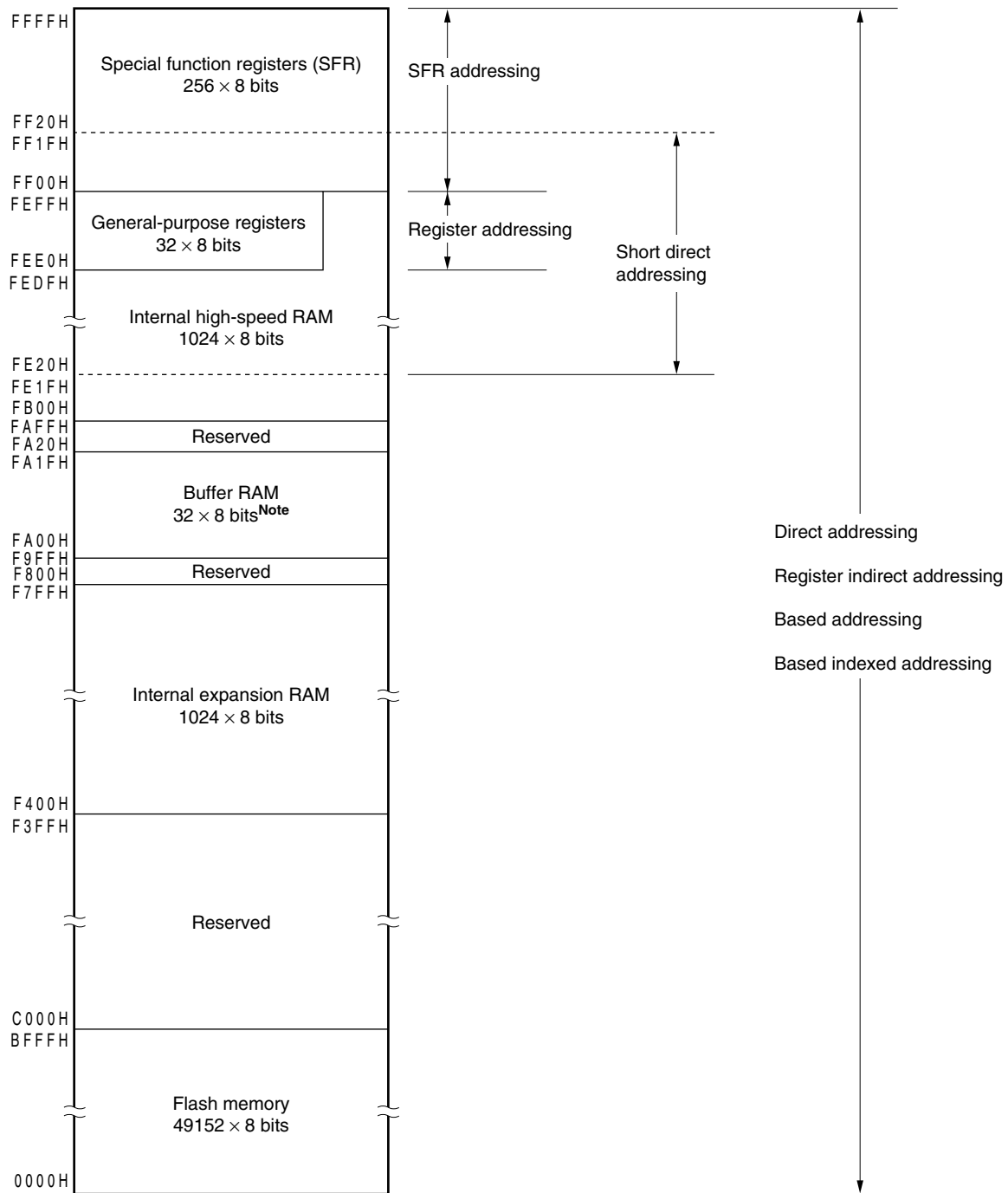
Figure 3-16. Correspondence Between Data Memory and Addressing ( \mu PD78F0514A, 78F0524A, 78F0534A, 78F0544A)
