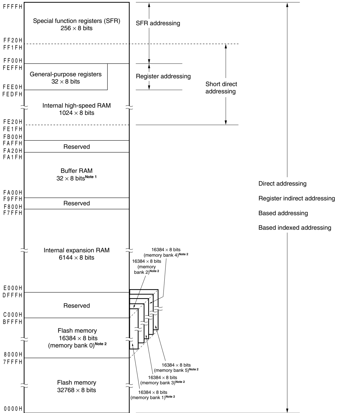
Figure 3-19. Correspondence Between Data Memory and Addressing ( \mu PD78F0527A, 78F0537A, 78F0547A, 78F0527DA, 78F0537DA, 78F0547DA)
