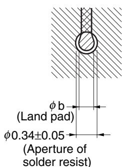
DETAIL OF (C) PART
