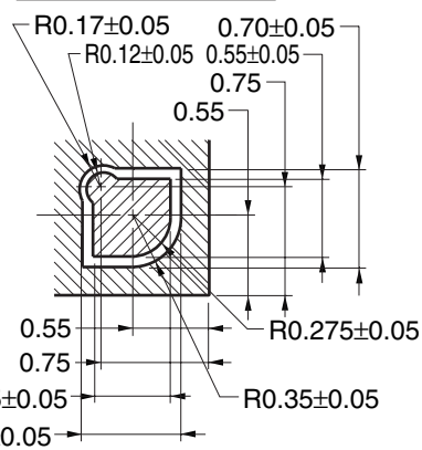
DETAIL OF (E) PART
