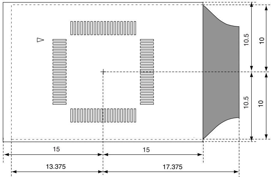
Figure B-10. For 64-Pin GK Package
