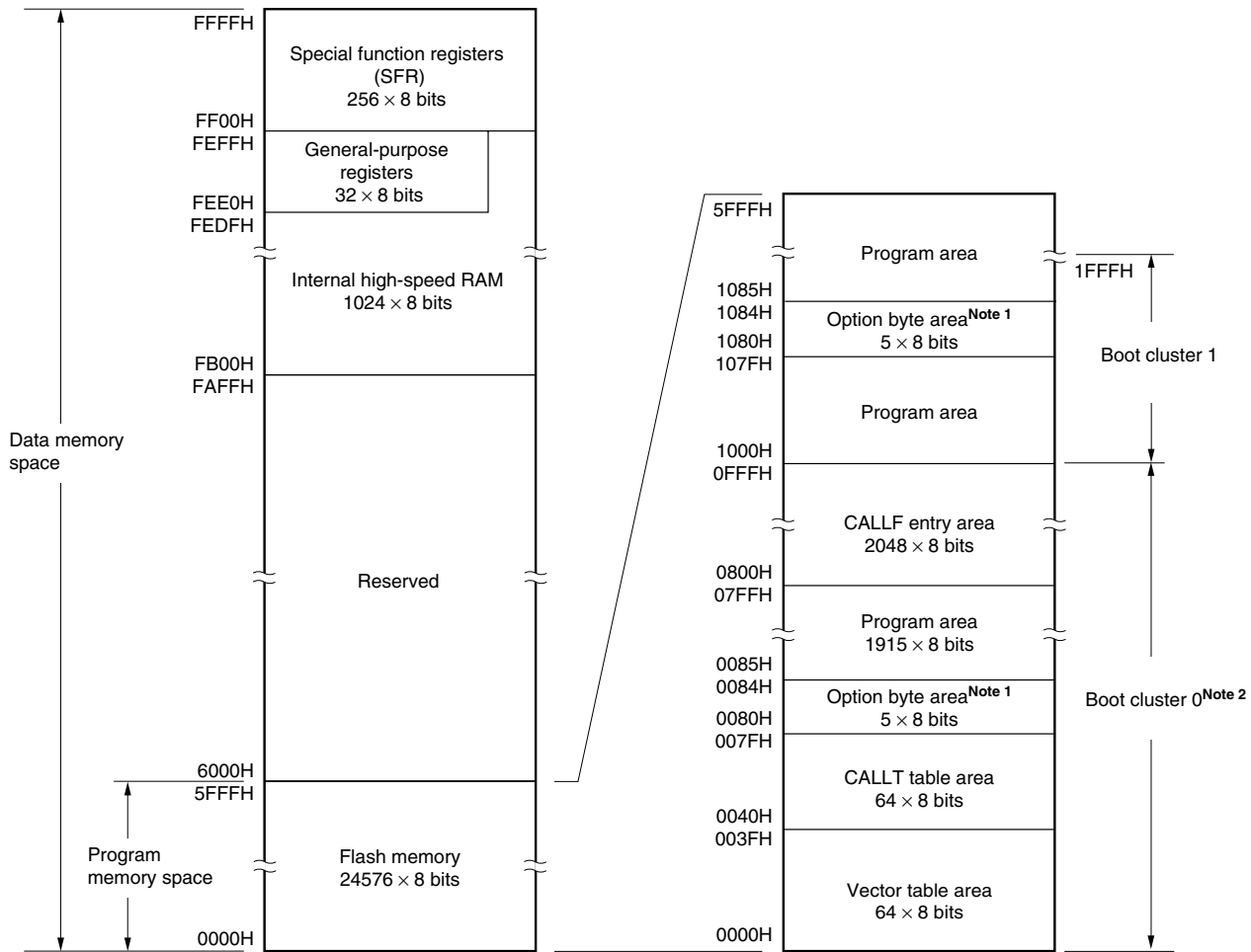
Figure 3-3. Memory Map ( \mu PD78F0502A, 78F0512A, 78F0522A, 78F0532A)
