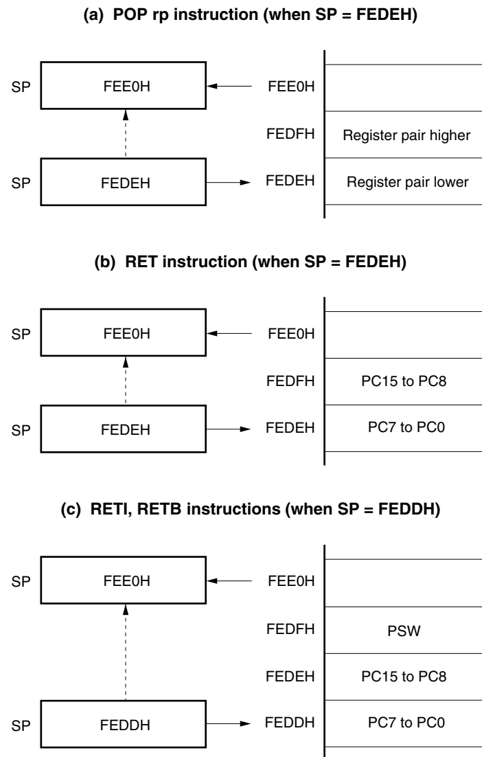
Figure 3-24. Data to Be Restored from Stack Memory
