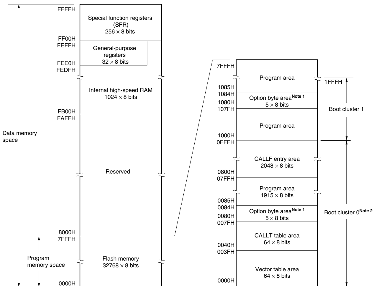
Figure 3-4. Memory Map ( \mu PD78F0503A, 78F0513A, 78F0523A, 78F0533A)
