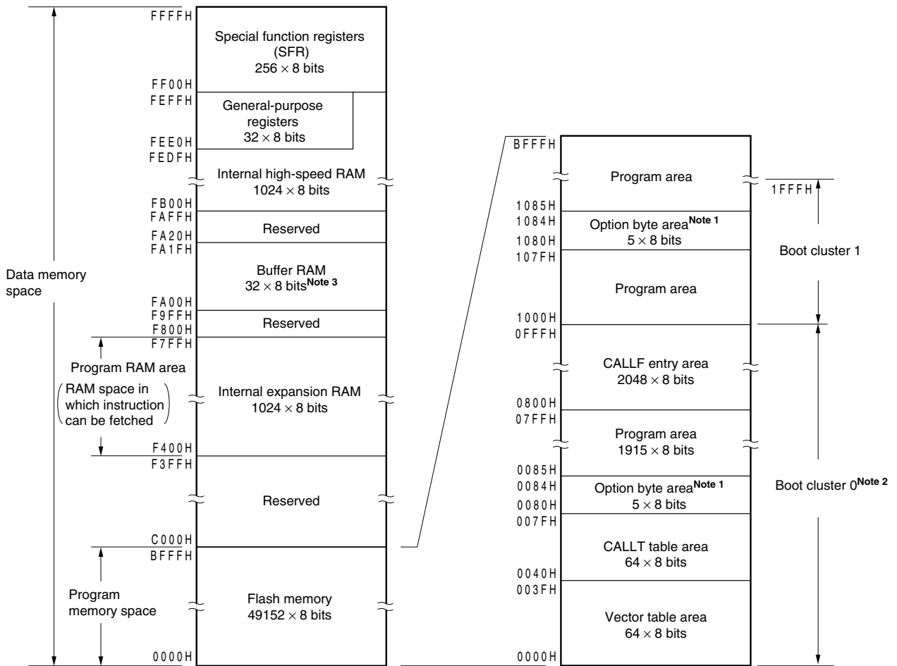
Figure 3-6. Memory Map ( \mu PD78F0514A, 78F0524A, 78F0534A, 78F0544A)
