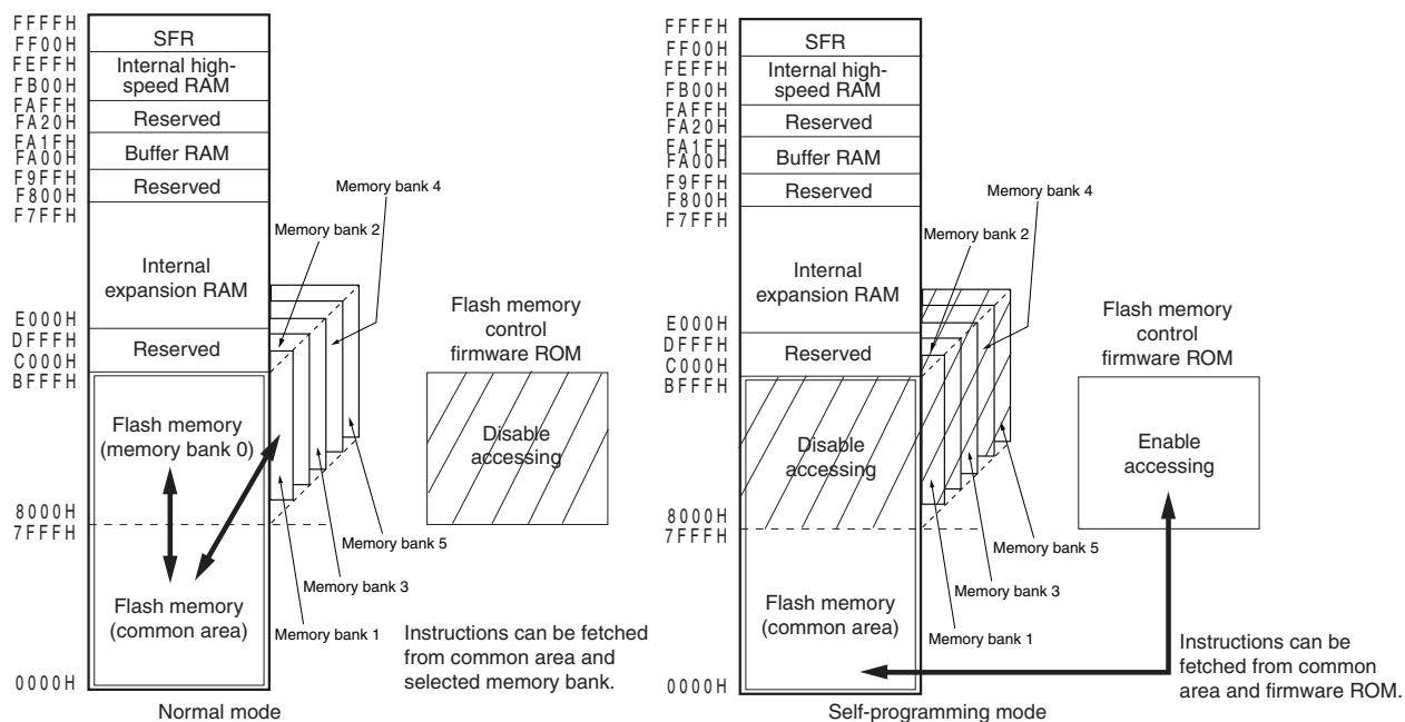
Figure 27-13. Operation Mode and Memory Map for Self-Programming ( \mu PD78F0547A)
