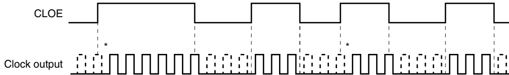
Figure 12-6. Remote Control Output Application Example
