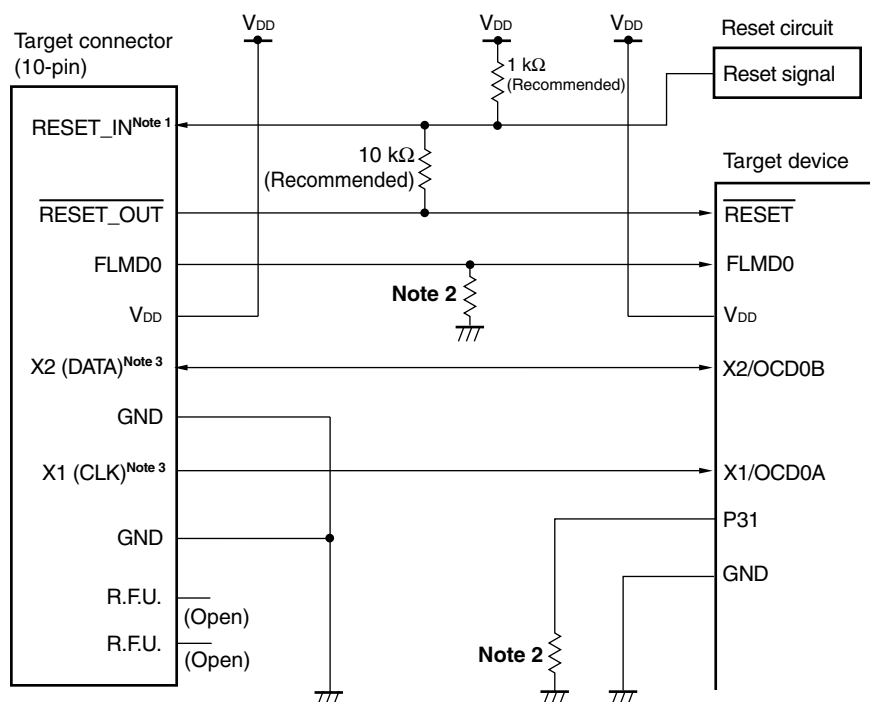
Figure 28-1. Connection Example of QB-78K0MINI or QB-MINI2 and \mu PD78F05xxDA (When OCD0A/X1 and OCD0B/X2 Are Used)
