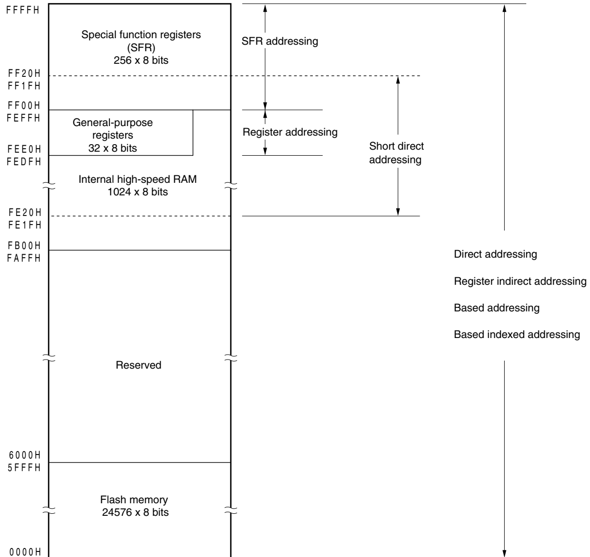
Figure 3-14. Correspondence Between Data Memory and Addressing ( \mu PD78F0502A, 78F0512A, 78F0522A, 78F0532A)
