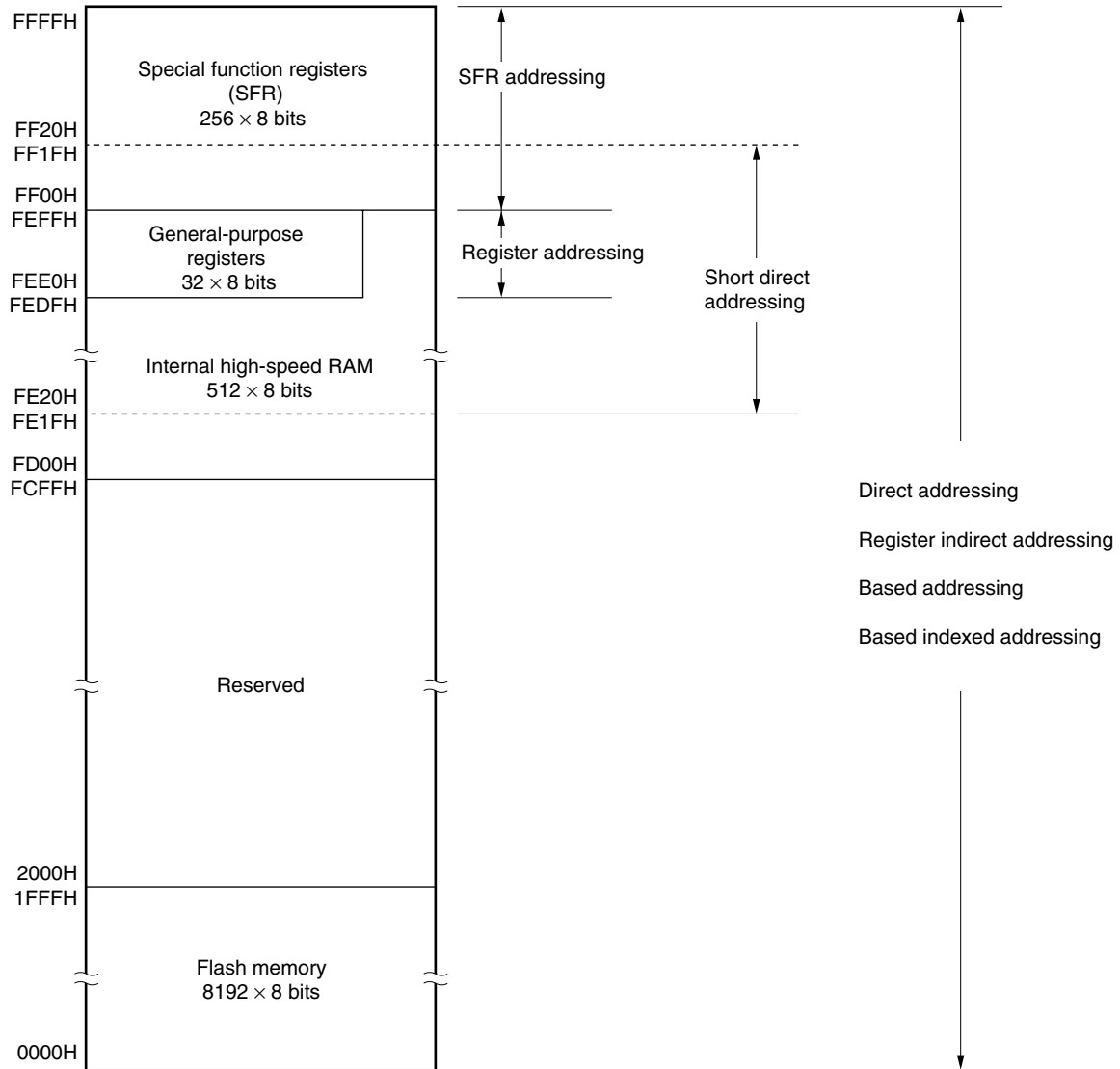
Figure 3-12. Correspondence Between Data Memory and Addressing ( \mu PD78F0500A)
