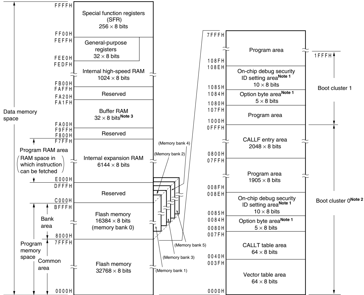
Figure 3-11. Memory Map ( \mu PD78F0527DA, 78F0537DA, 78F0547DA)
