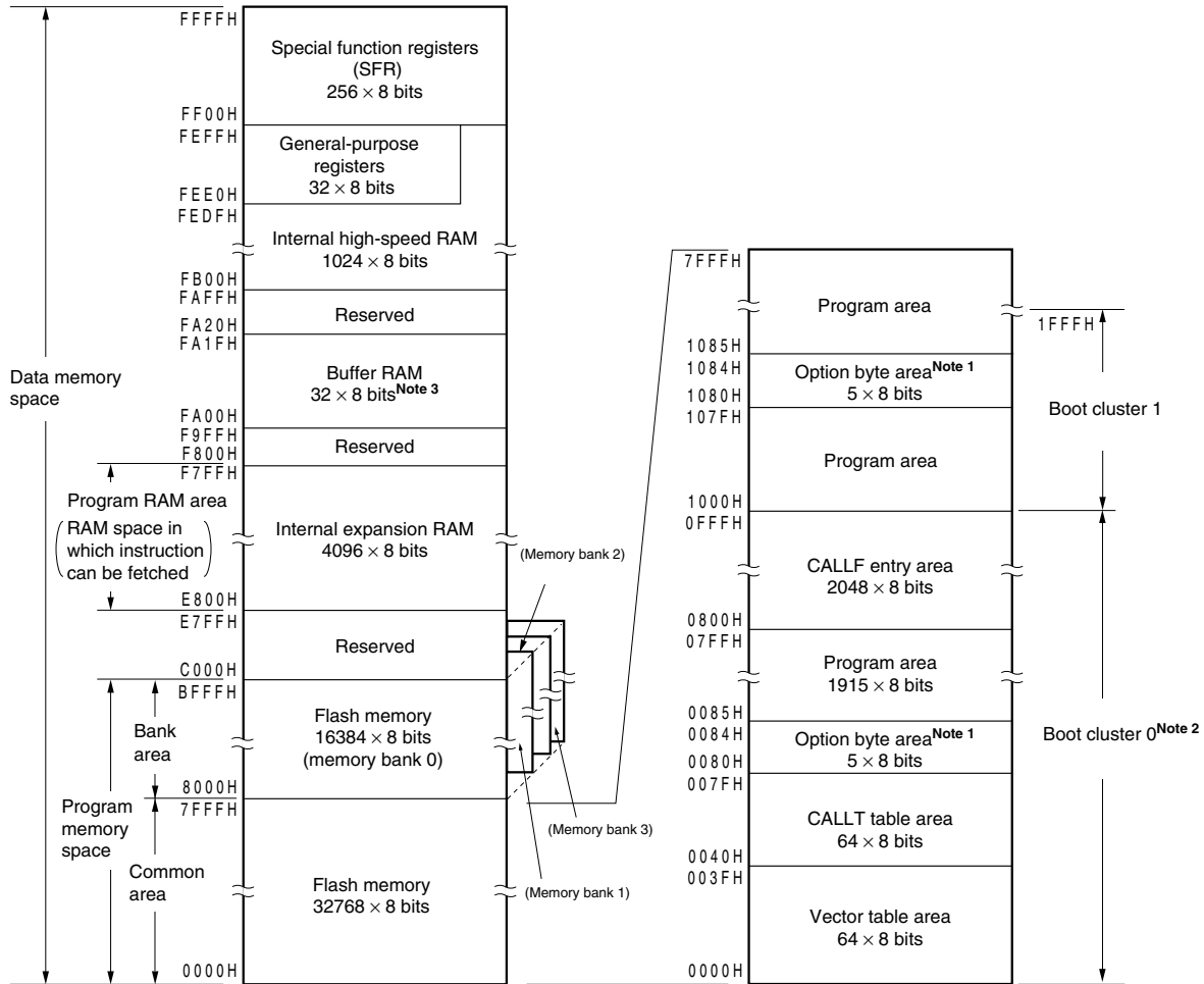
Figure 3-9. Memory Map ( \mu PD78F0526A, 78F0536A, 78F0546A)
