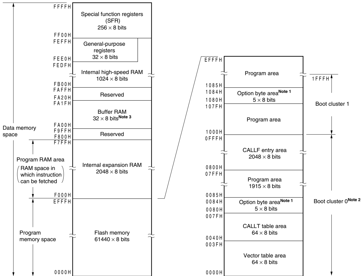
Figure 3-7. Memory Map ( \mu PD78F0515A, 78F0525A, 78F0535A, 78F0545A)
