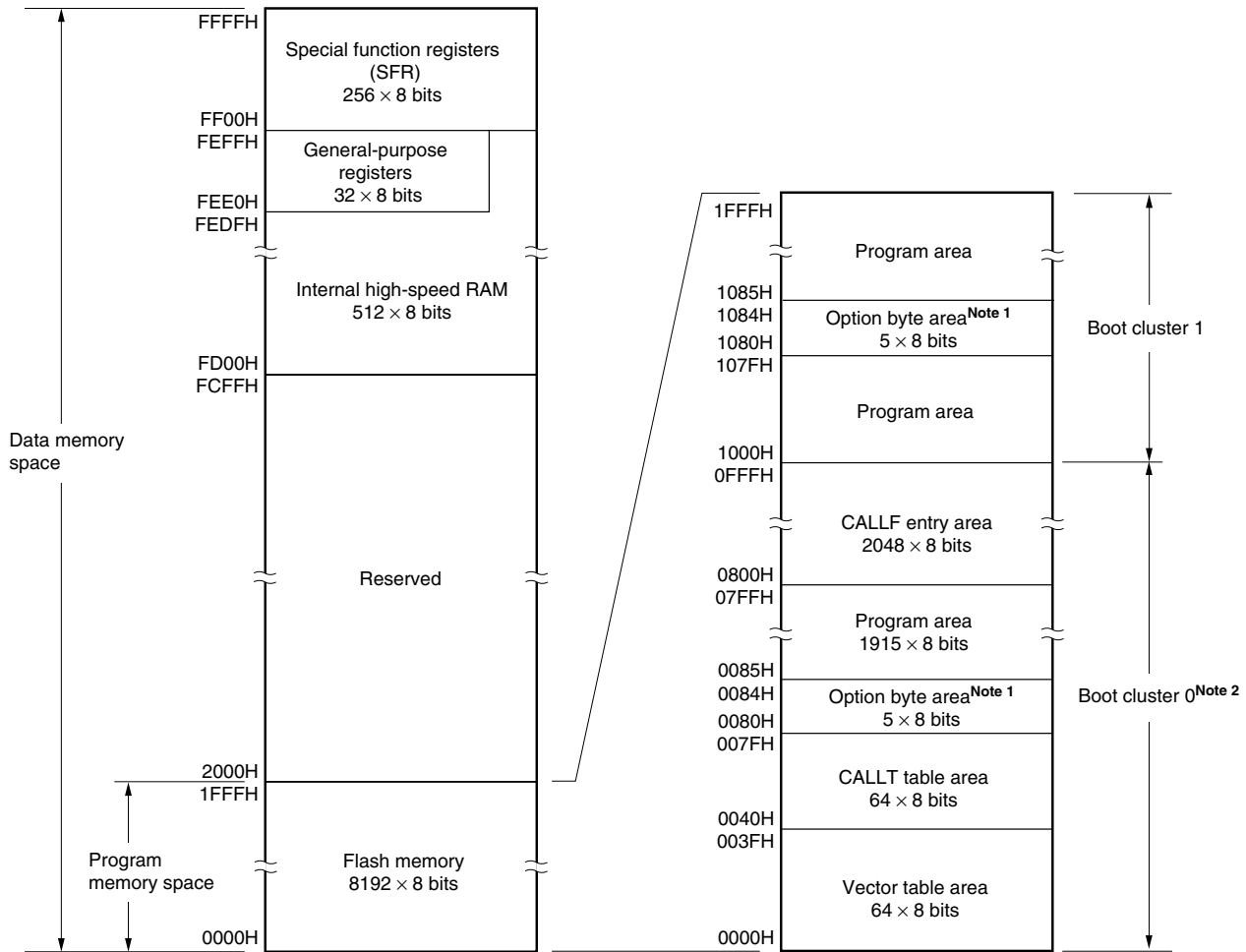
Figure 3-1. Memory Map ( \mu PD78F0500A)
