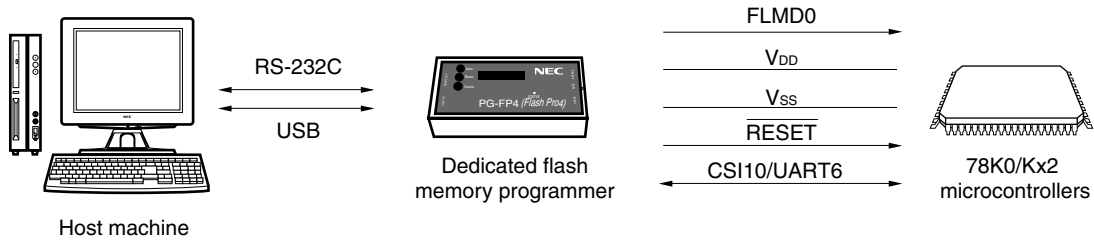
Figure 27-3. Environment for Writing Program to Flash Memory
