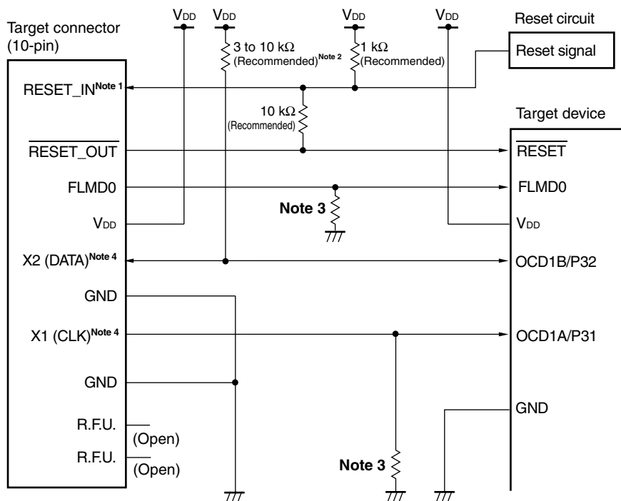
Figure 28-2. Connection Example of QB-78K0MINI or QB-MINI2 and μPD78F05xxDA (When OCD1A/P31 and OCD1B/P32 Are Used)
