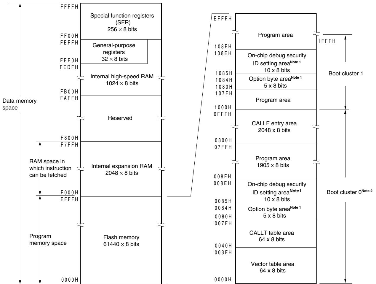
Figure 3-8. Memory Map ( \mu PD78F0515DA)
