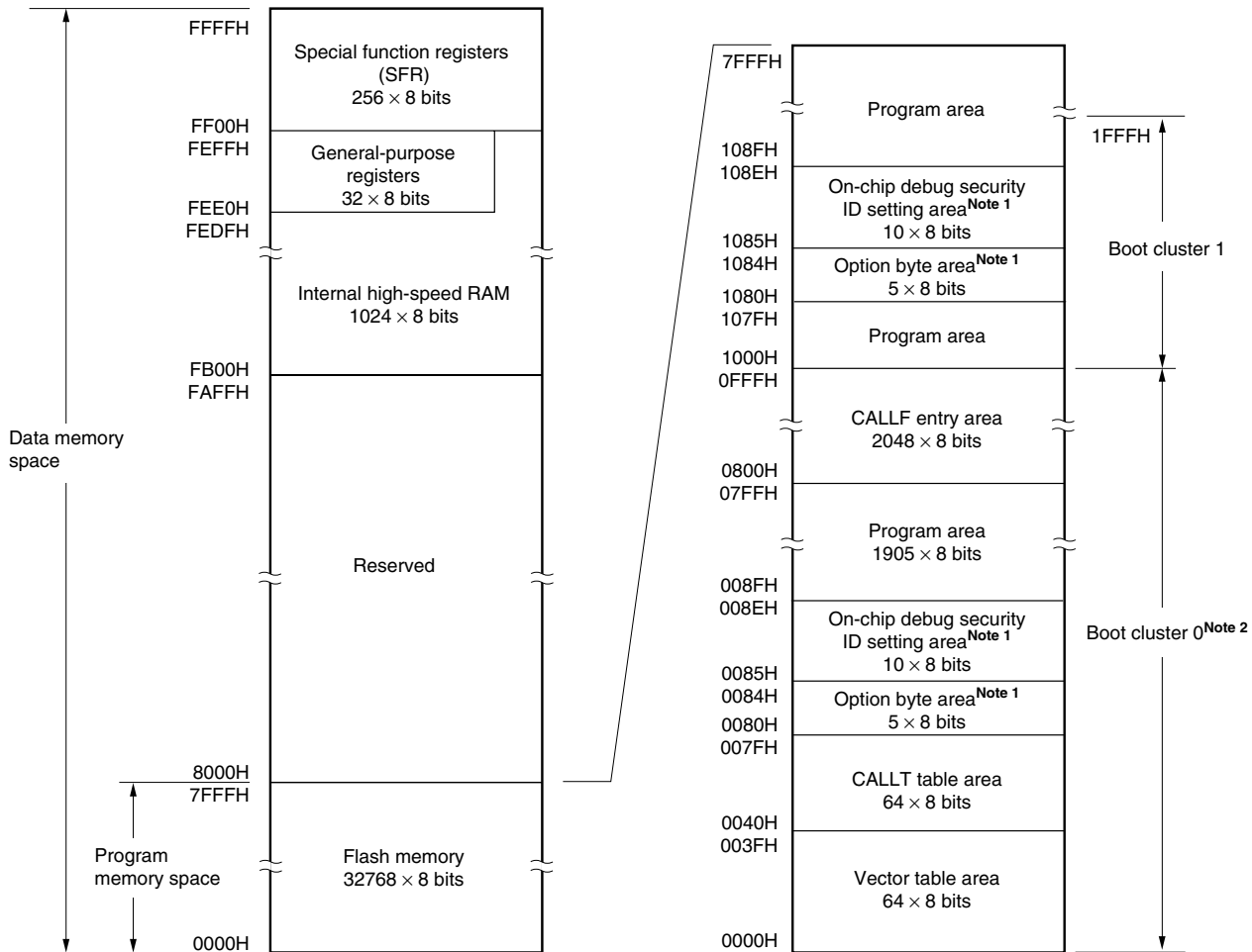
Figure 3-5. Memory Map ( \mu PD78F0503DA, 78F0513DA)
