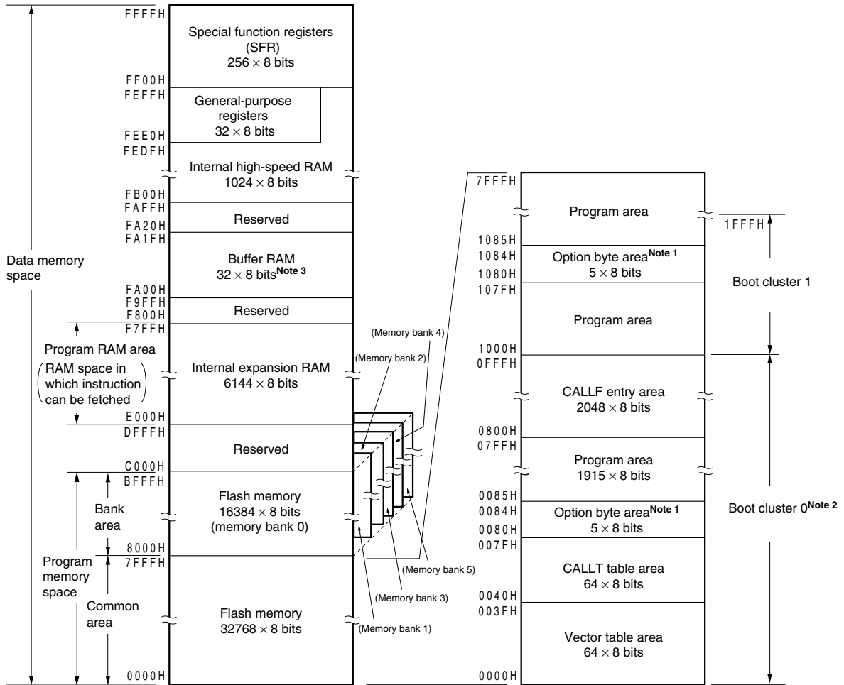
Figure 3-10. Memory Map ( \mu PD78F0527A, 78F0537A, 78F0547A)
