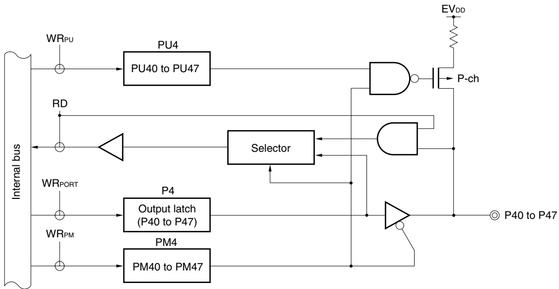
Figure 5-15. Block Diagram of P40 to P47
