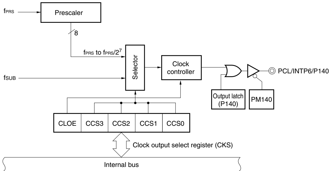
Figure 12-1. Block Diagram of Clock Output/Buzzer Output Controller (48-pin products of 78K0/KC2, 78K0/KD2)
