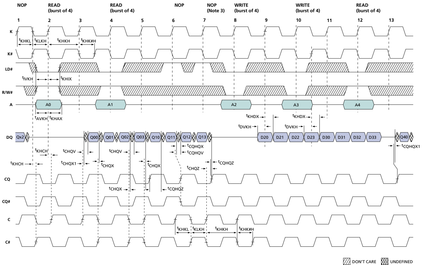
Figure 6: READ/WRITE Timing
