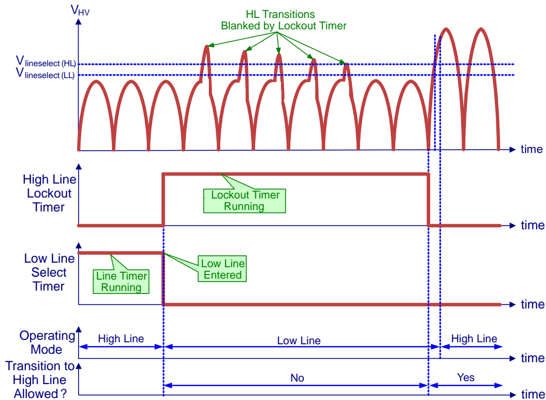
Figure 25. Lockout Timer Operation (Version C5 Only)
