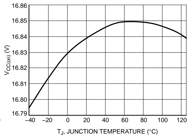
Figure 36. V CC(on) (Version C/D) vs. Temperature
