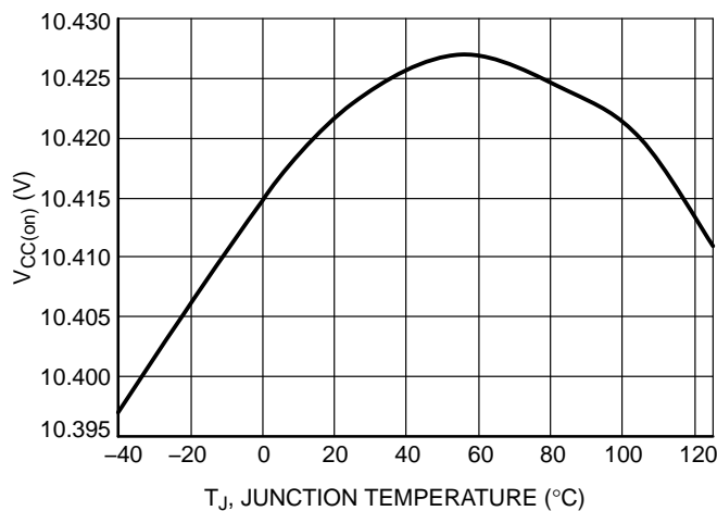
Figure 35. V CC(on) (Version A/B) vs. Temperature
