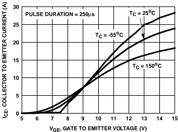
FIGURE 13. TRANSFER CHARACTERISTIC
