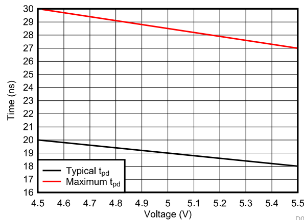
Figure 1. Propagation Delay Over Operating Voltage Range, T_A = 25^\circ\text{C}
