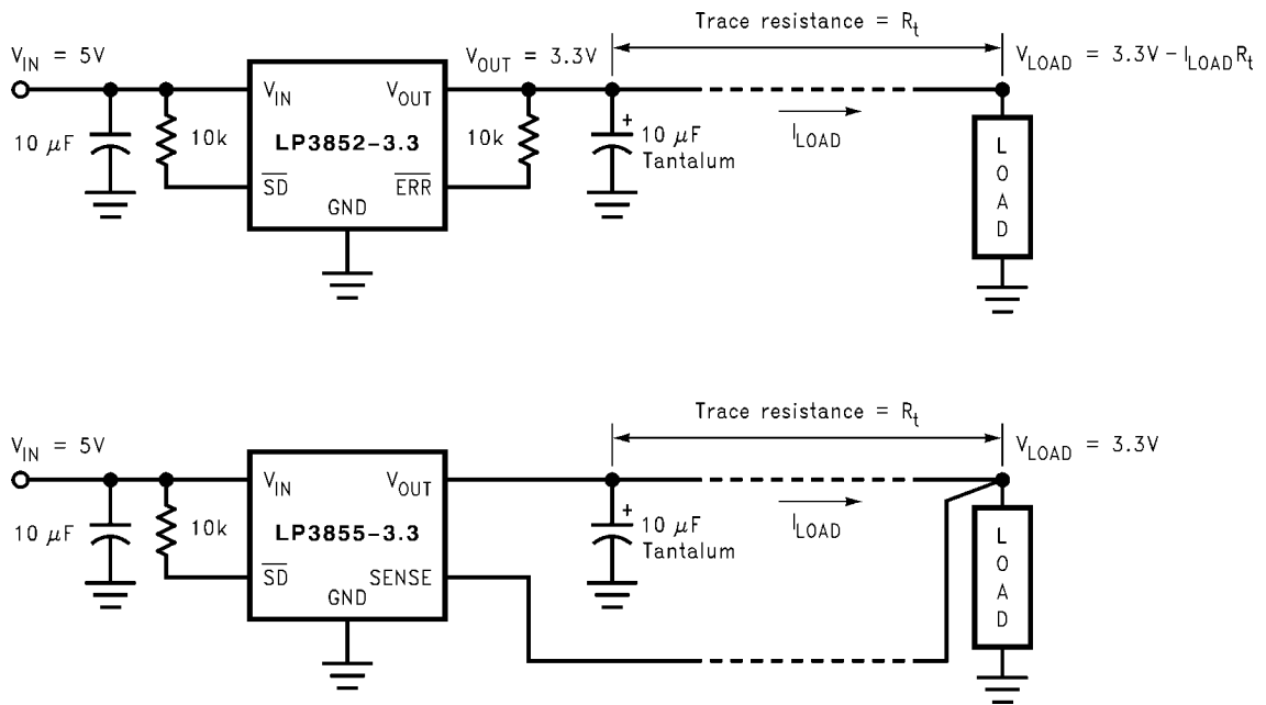
FIGURE 4. Improving remote load regulation using LP3855
