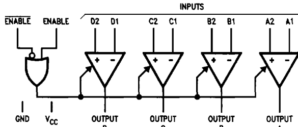
FIGURE 1. Logic Symbol
