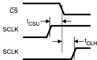
SCLK and \overline{\text{CS}} Timing Parameters
