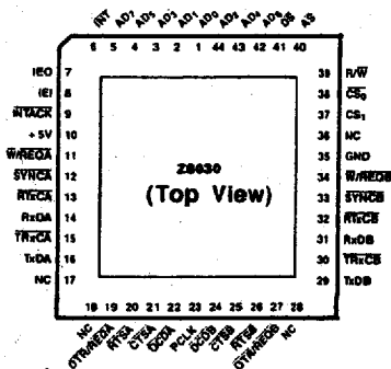
Figure 2d. Chip Carrier Pin Assignments, Z8030
