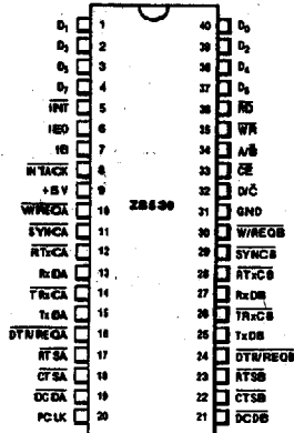
Figure 2a. DIP Pin Assignments, Z8830
