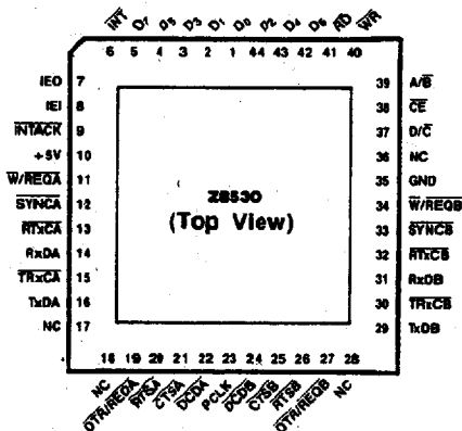
Figure 2c. Chip Carrier Pin Assignments, Z8830
