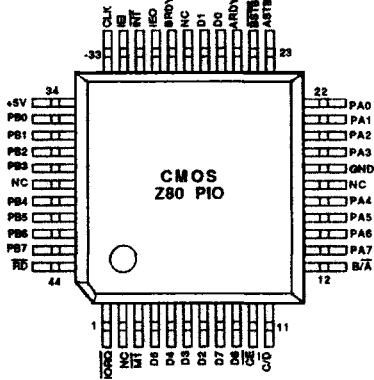
Figure 2c. 44-pin Quad Flat Pack Pin Assignments.
