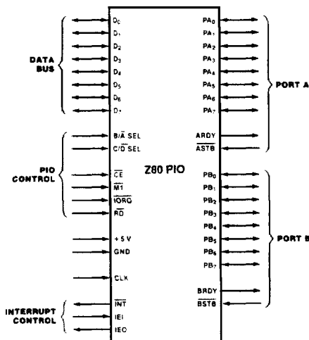
Figure 1. Pin Functions
