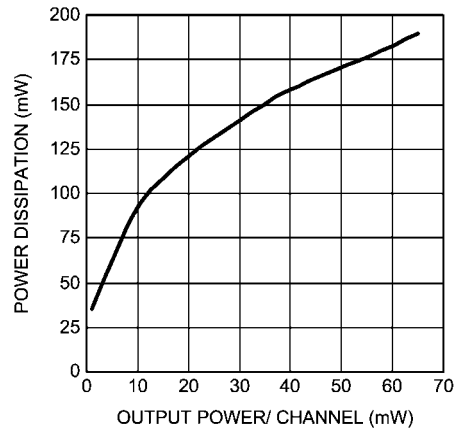
Power Dissipation vs Output Power V_{DD} = 3\text{V} , R_L = 32\Omega , f = 1\text{kHz}
