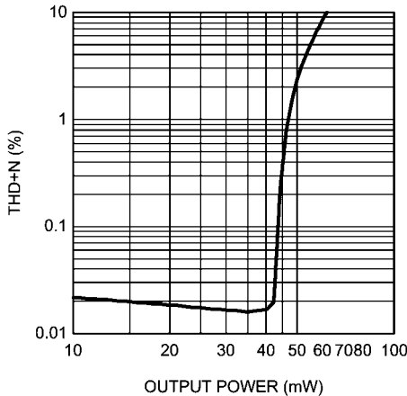
THD+N vs Output Power V_{DD} = 3.6V, R_L = 16\Omega f = 1kHz, 22kHz BW, one channel enabled
