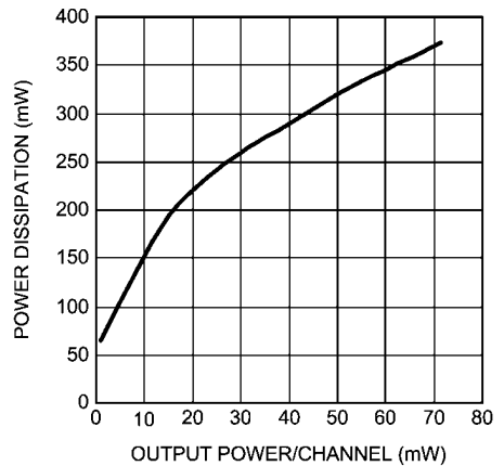
Power Dissipation vs Output Power V_{DD} = 5\text{V} , R_L = 32\Omega , f = 1\text{kHz}
