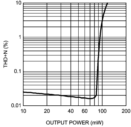
THD+N vs Output Power V_{DD} = 3V, R_L = 16\Omega f = 1kHz, 22kHz BW, one channel enabled
