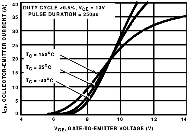
FIGURE 1. TRANSFER CHARACTERISTICS
