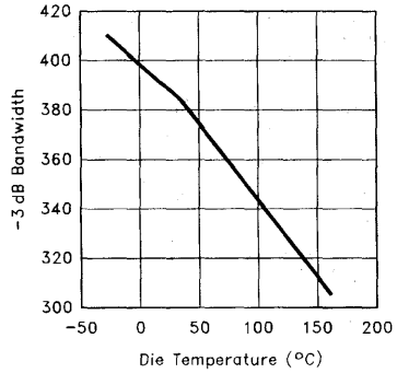
Bandwidth vs Die Temperature
