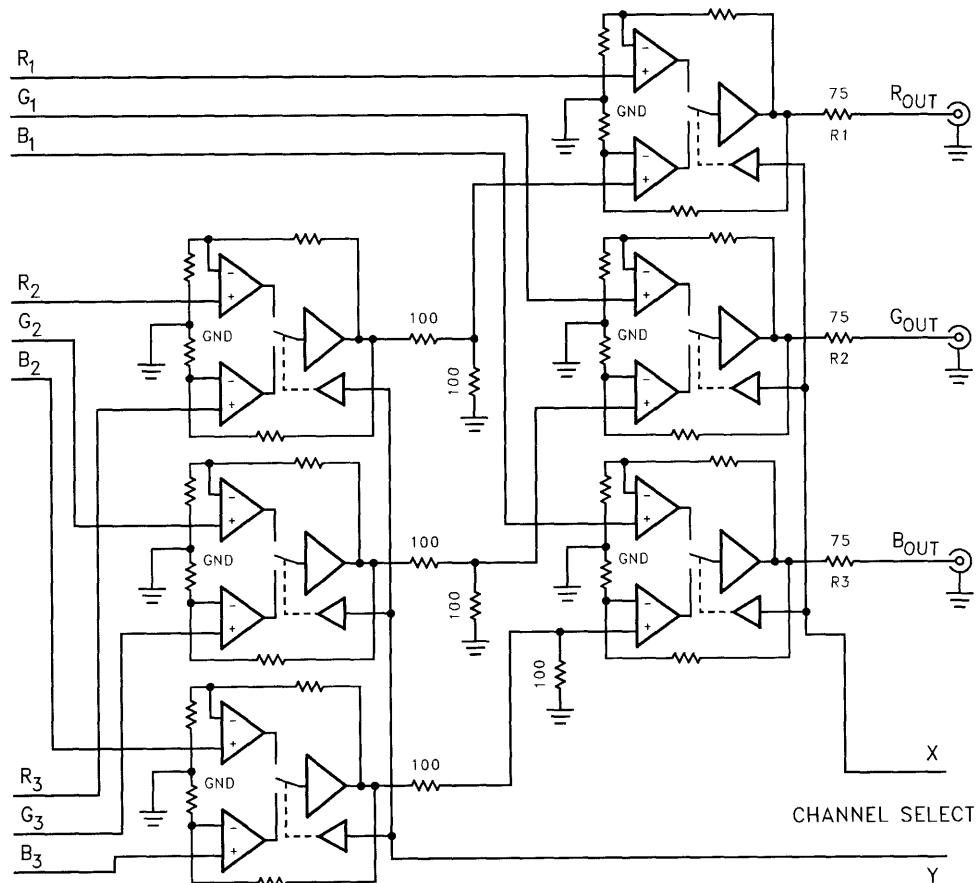
Figure 4. Typical Connection for a 3:1 Component Video Multiplexer
