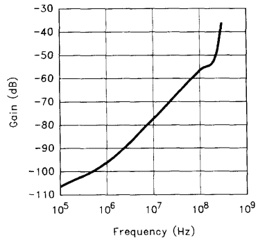
Channel-Channel Isolation
