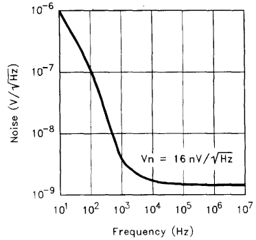
Input Voltage Noise over Frequency
