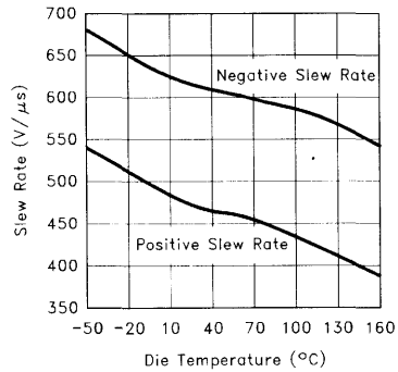
Slew Rate vs Die Temperature
