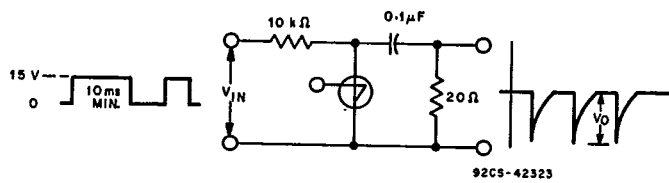
Fig. 14—Peak pulse voltage test circuit and waveforms.
