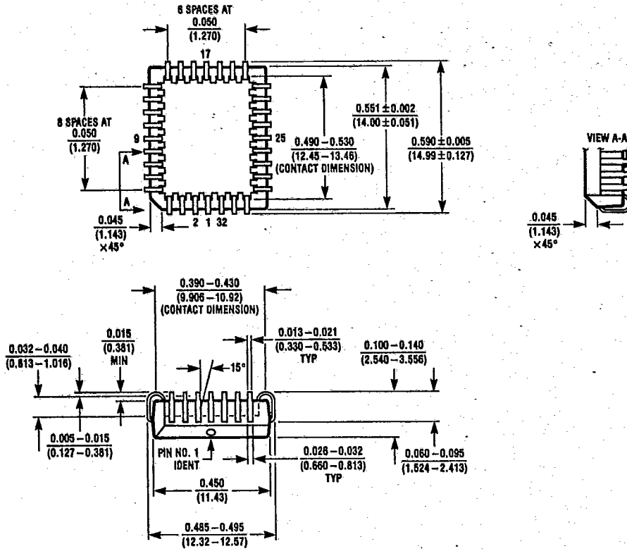
32-Lead PLCC Package Order Number NMC27C256
