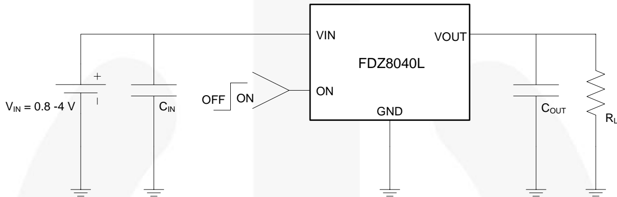
Figure 21. Typical Application
