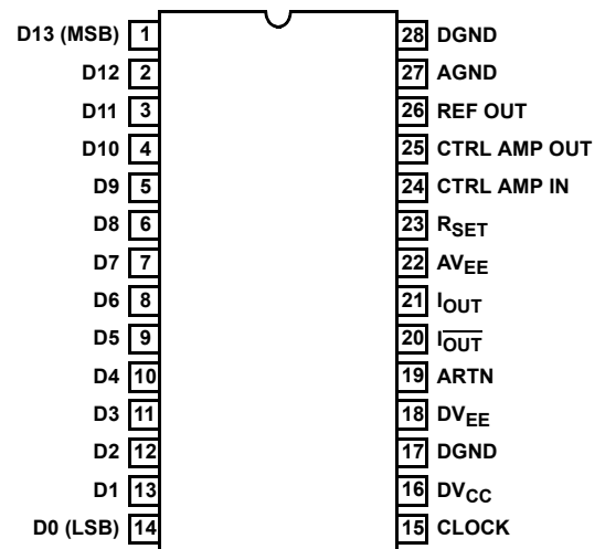
HI5741 (PDIP, SOIC) TOP VIEW
