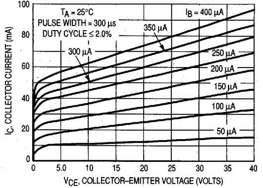
Figure 7. Collector Characteristics
