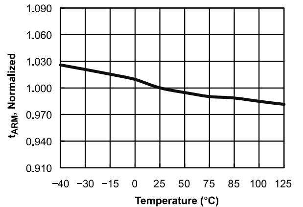
Figure 14. Gate Re-arming Time for Slope Detection (t ARM ) vs. Temperature
