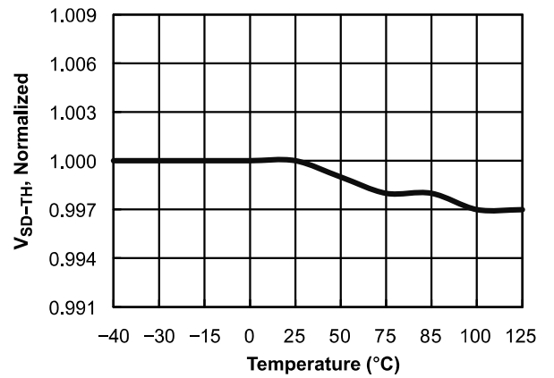
Figure 12. Shut-Down Threshold Voltage (V SD-TH ) vs. Temperature
