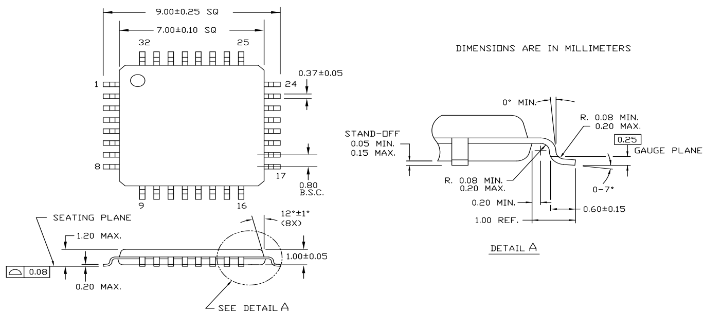
Figure 14. 32-Pin Thin Plastic Quad Flat Pack, 51-85063
