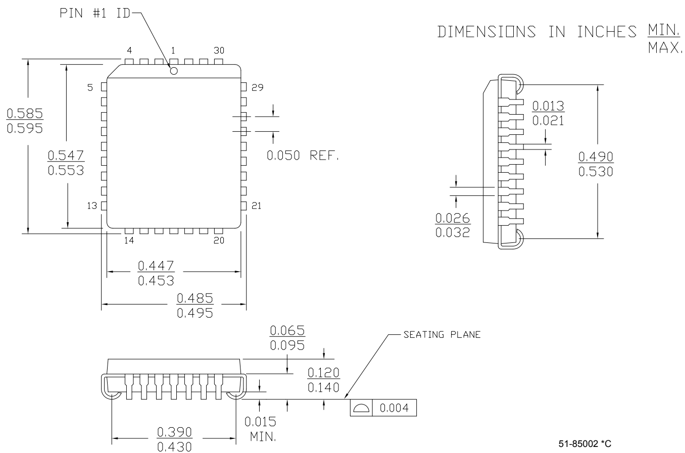
Figure 15. 32-Pin Plastic Leaded Chip Carrier, 51-85002
