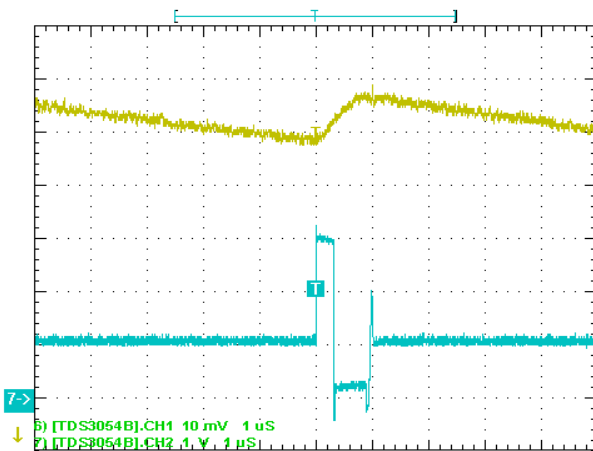
Ripple in DCM: Fripple = 145kHz, Vin = 2.85V, Vout = 0.85V, Iout = 10mA Ripple = 10mV (worst case), 1 \mu s/DIV
