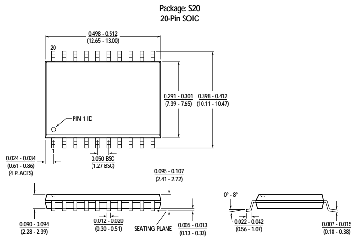
Package: S20 20-Pin SOIC
