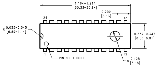
24 Lead Ceramic Dual-In-Line Package (0.400" Wide) (D) Package Number J24E
