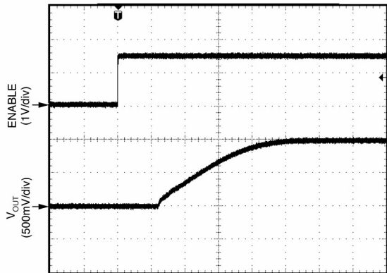
Turn-On Transient
