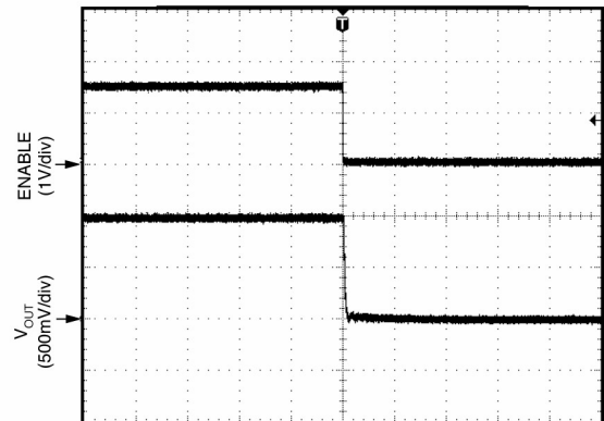
Turn-Off Transient
