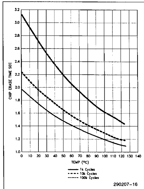
Figure 10. Typical Erase Time at 12V
