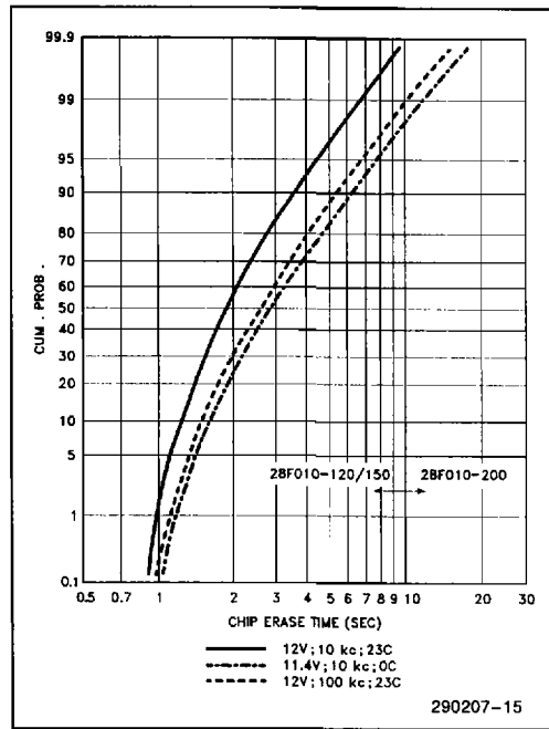
Figure 9. Typical Erase Capability
