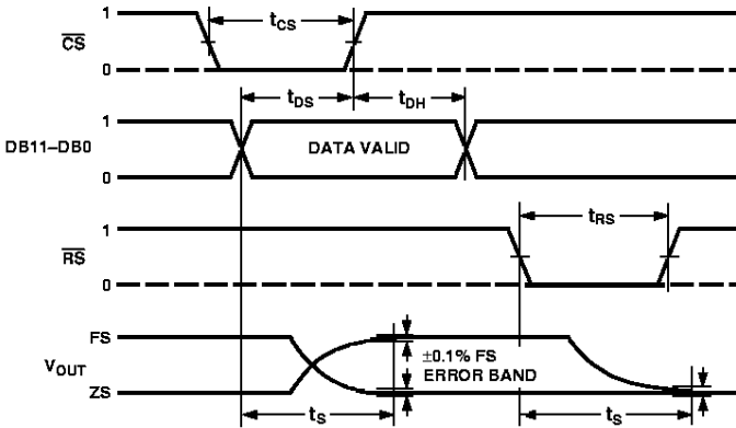
Figure 3. Timing Diagram
