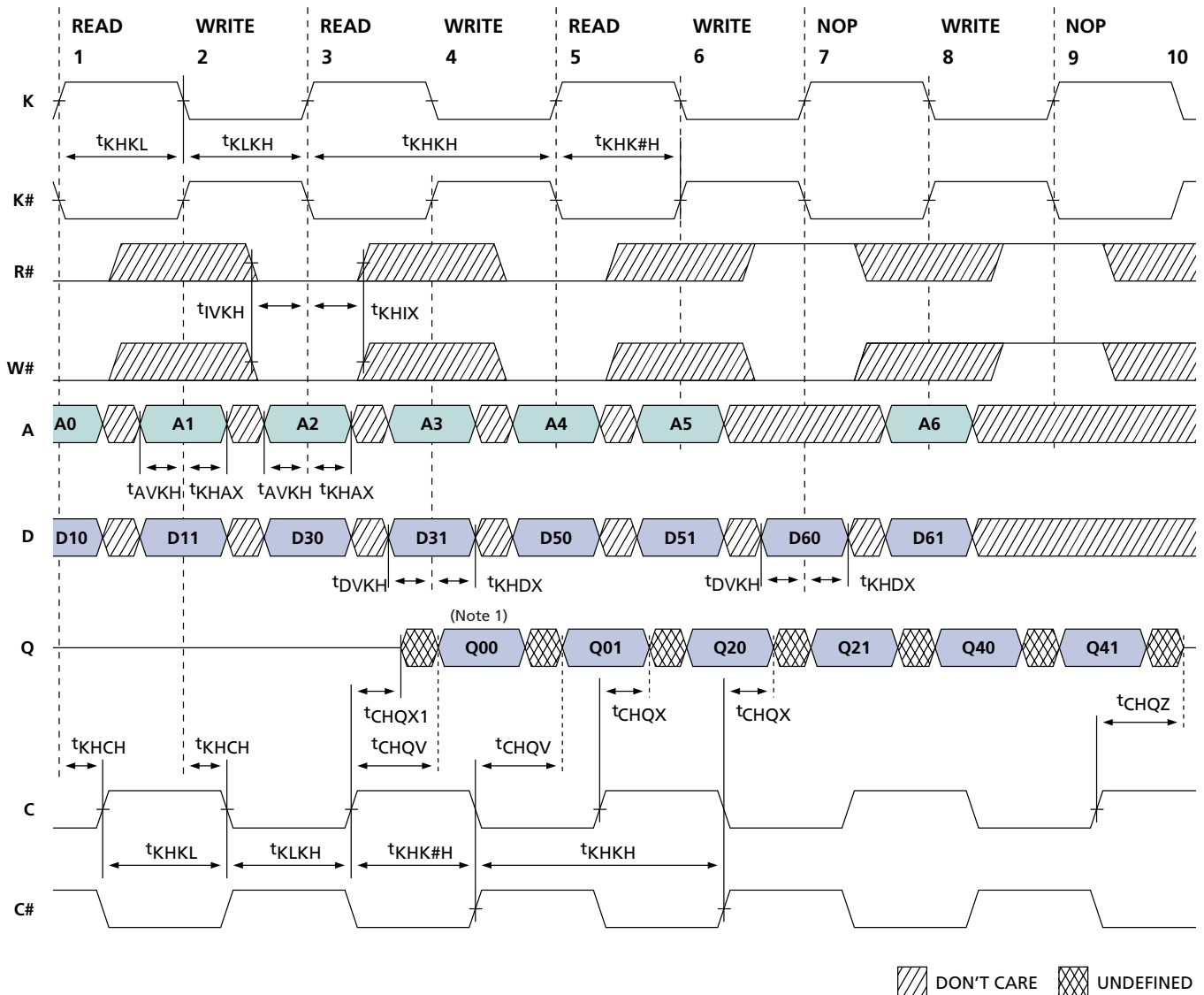
Figure 6: READ/WRITE Timing
