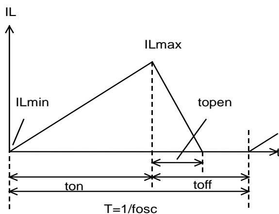
Discontinuous mode
