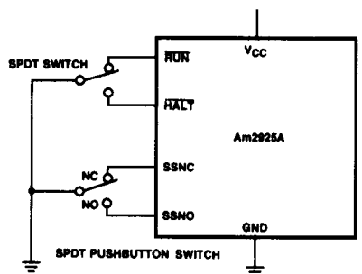
Figure 6. Switch Connection for RUN/HALT and Single Step
