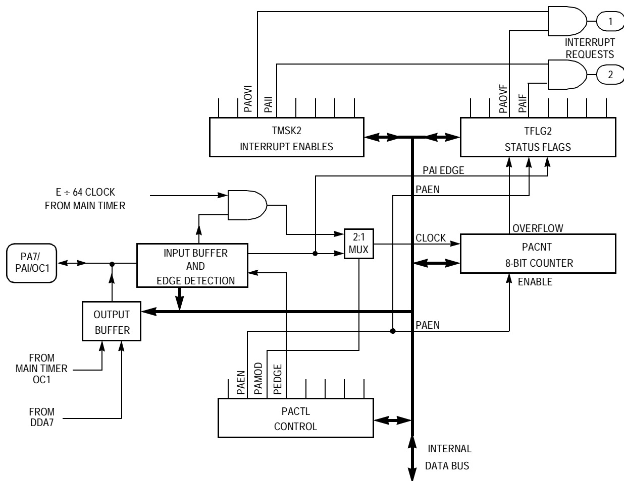
Figure 9-21. Pulse Accumulator
