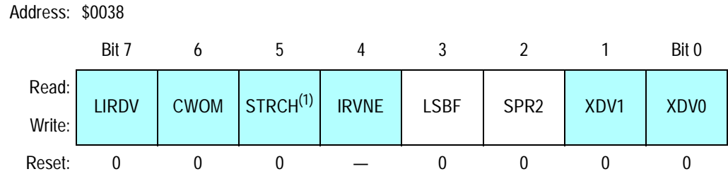
Figure 8-7. System Configuration Options 2 Register (OPT2)
