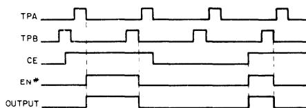
Fig. 3 — Timing diagram.
