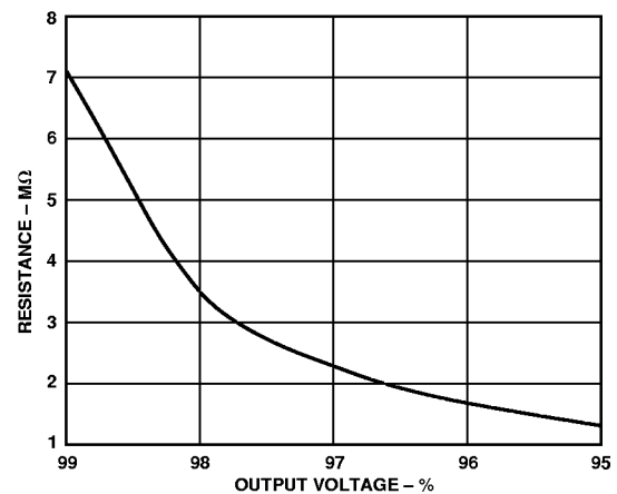
Figure 24. External Resistor Value for Reducing Output Voltage
