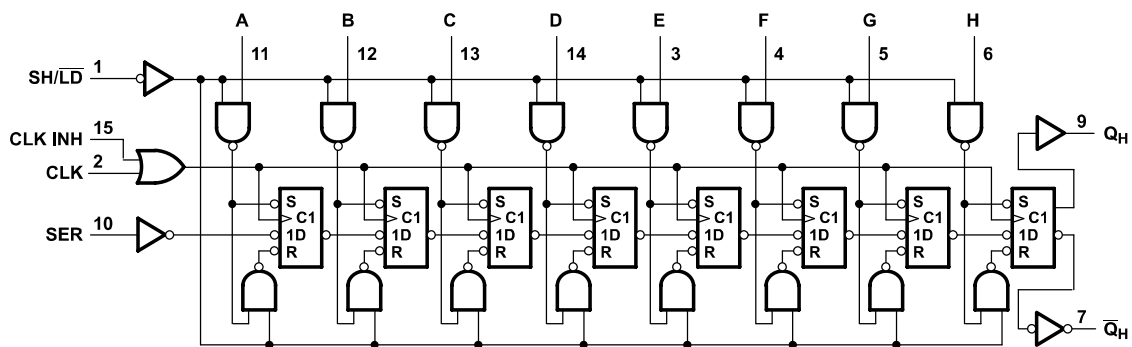
Figure 3. Logic Diagram Positive Logic
