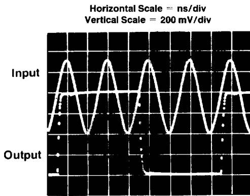
25 MHz Operation
