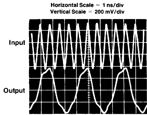
1.2 GHz Operation
