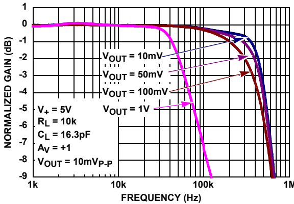
FIGURE 3. GAIN vs FREQUENCY vs V_{OUT} , R_L = 10k
