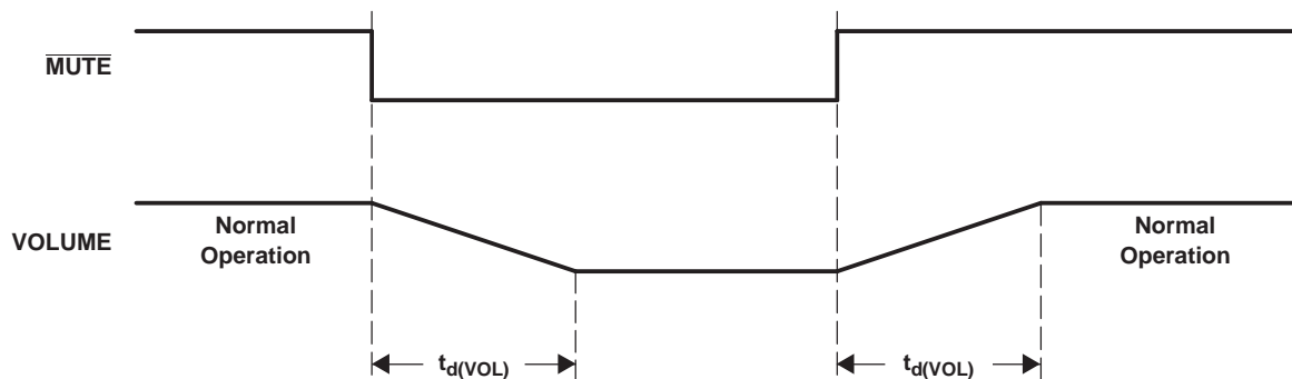
Figure 4-7. Mute Timing
