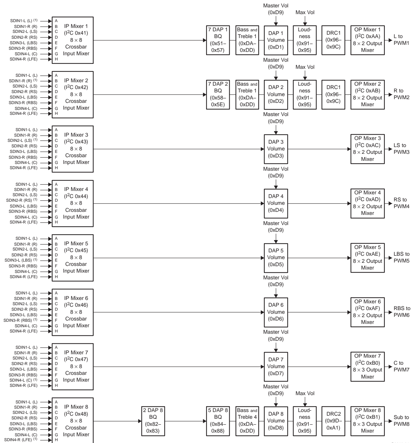
Figure 2-2. TAS5518C Architecture With I²C Registers ( f_s = 176.4 kHz or f_s = 192 kHz)
