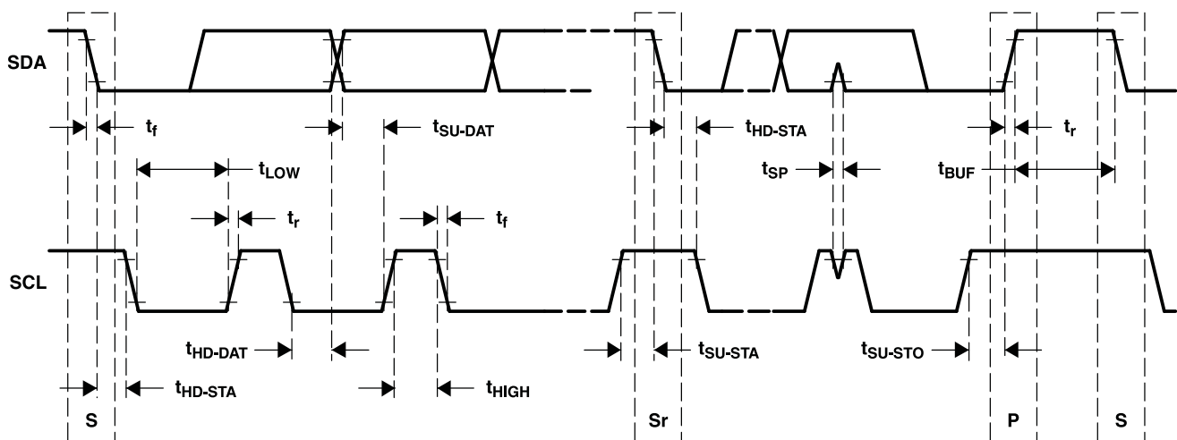
Figure 4-2. SCL and SDA Timing
