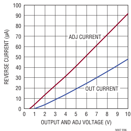
Figure 6. Reverse-Output Current
