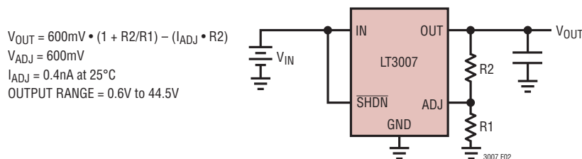
Figure 2. Adjustable Operation
