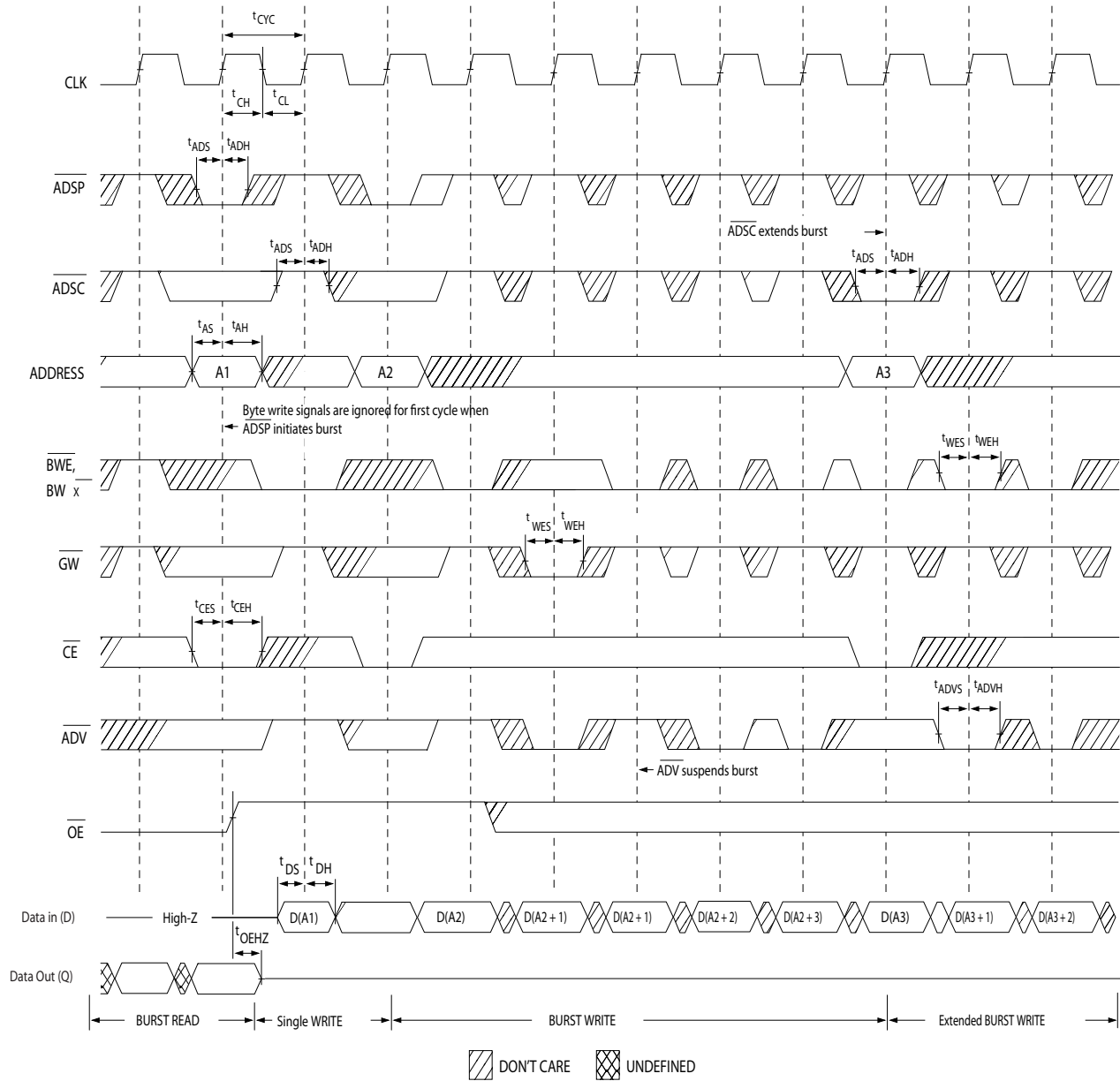
Figure 6. Write Cycle Timing [32, 33]
