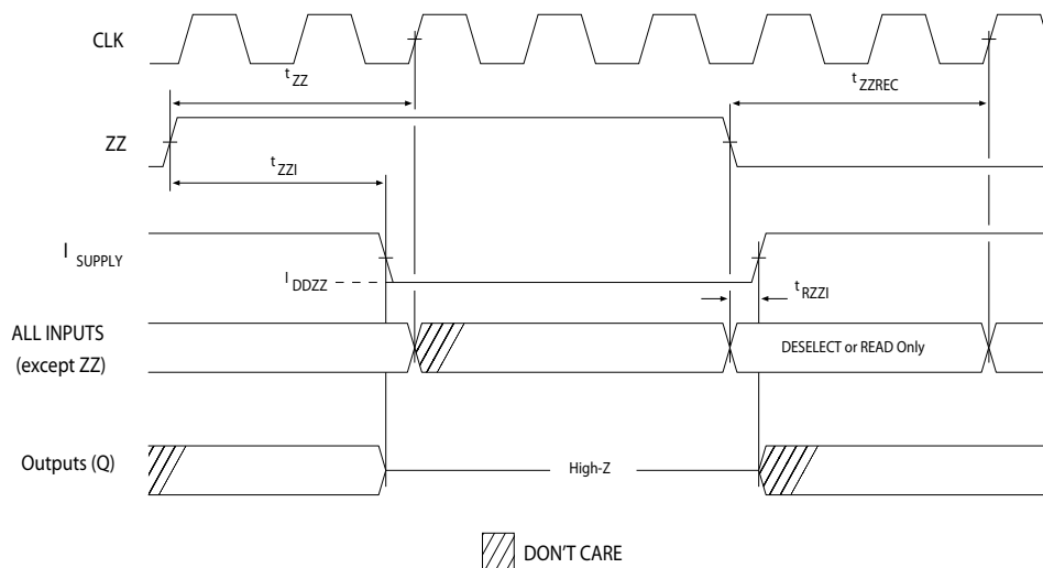
Figure 8. ZZ Mode Timing [37, 38]
