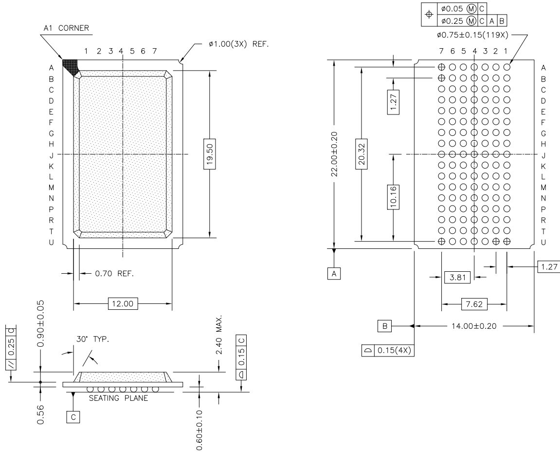
Figure 10. 119-ball BGA (14 × 22 × 2.4 mm), 51-85115
