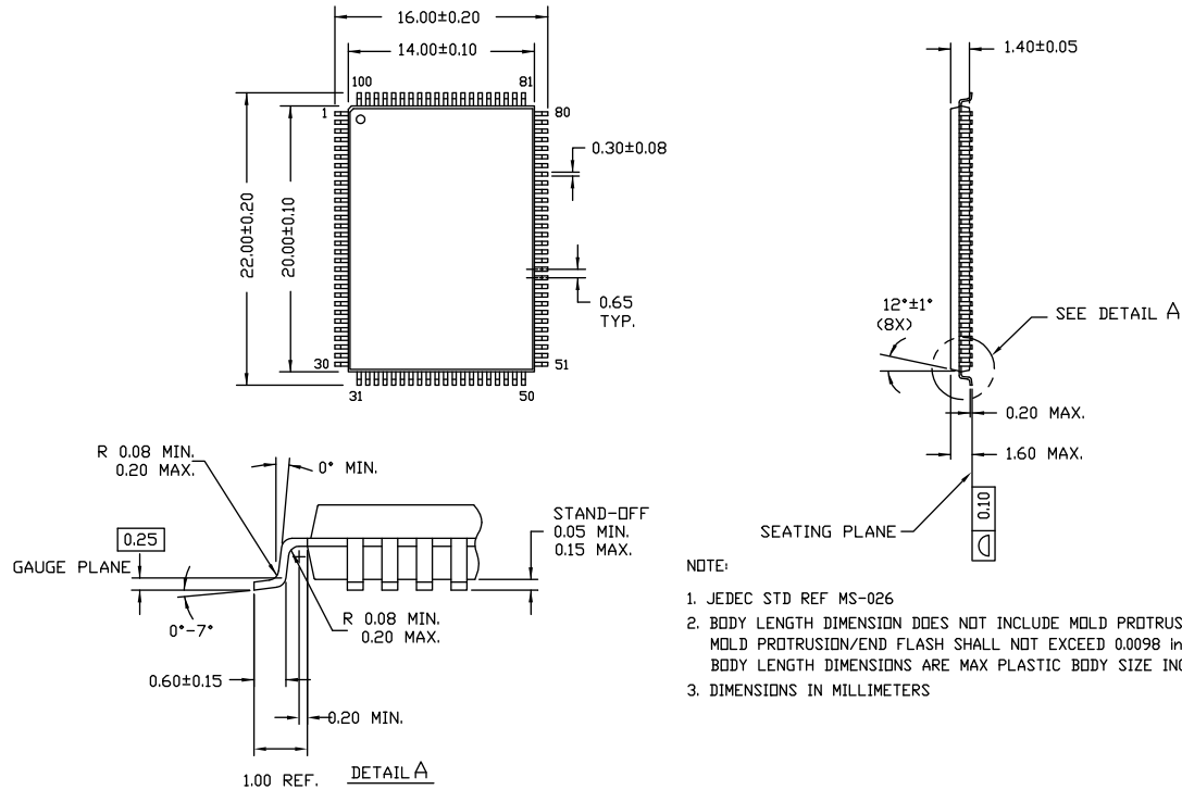
Figure 9. 100-pin Thin Plastic Quad Flat pack (14 × 20 × 1.4 mm), 51-85050
