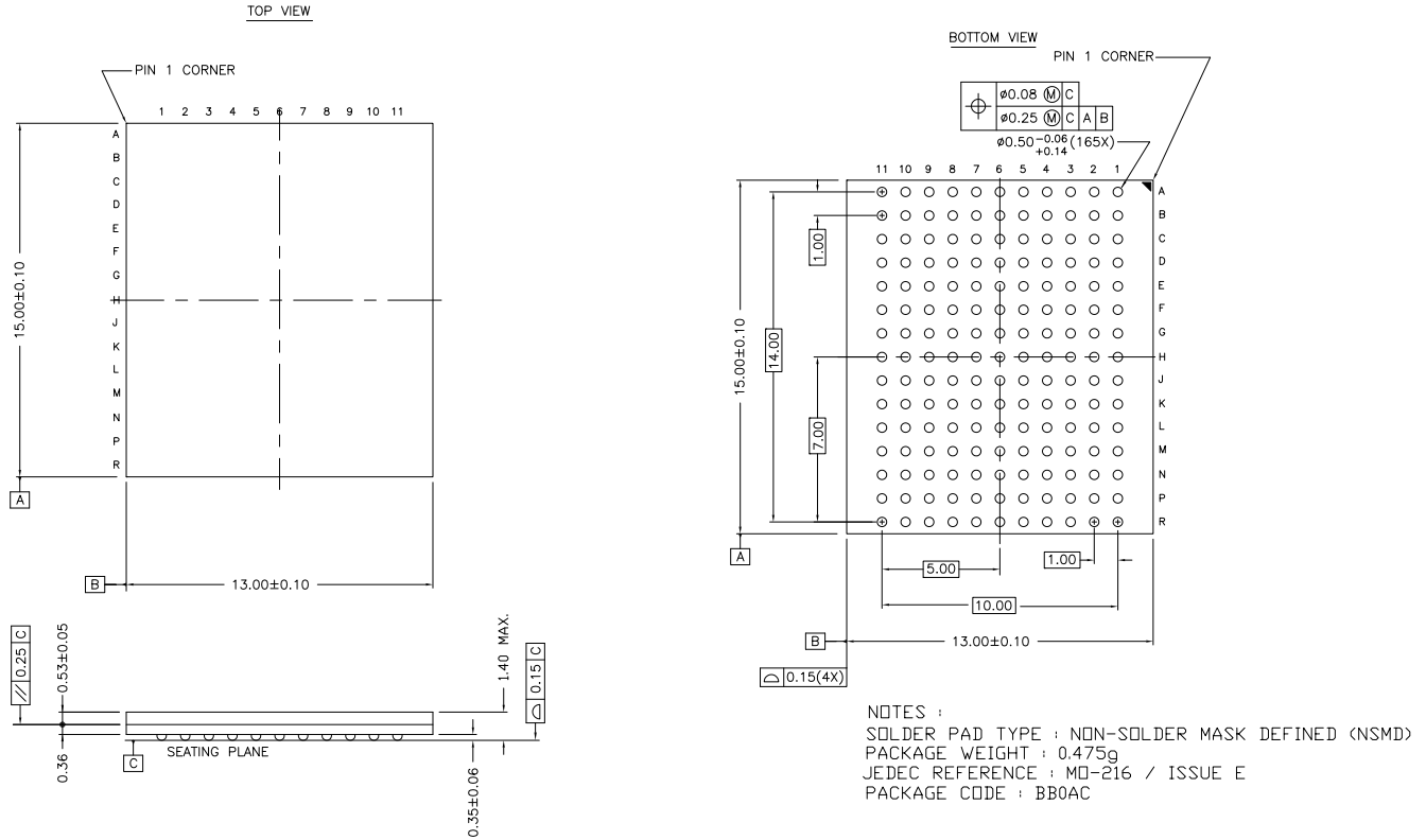
Figure 11. 165-ball FBGA (13 × 15 × 1.4 mm), 51-85180
