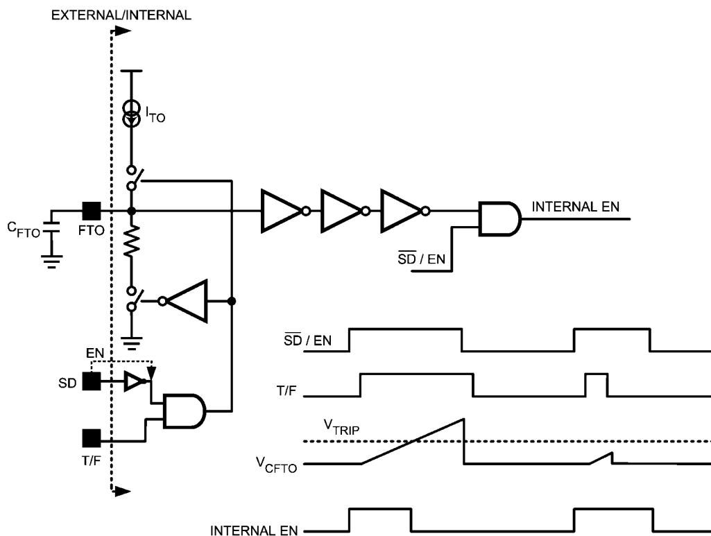
Flash Timeout Protection Diagram
