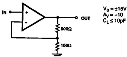
FIGURE 1. TEST CIRCUIT
