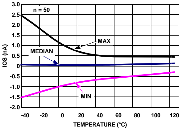
FIGURE 25. I_{OS} vs TEMPERATURE, V_S = \pm 2.5V
