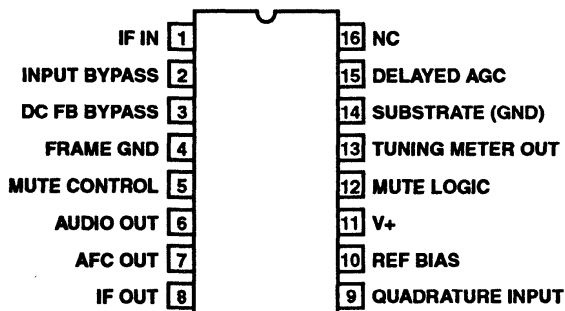
CA3089 (PDIP, CDIP) TOP VIEW
