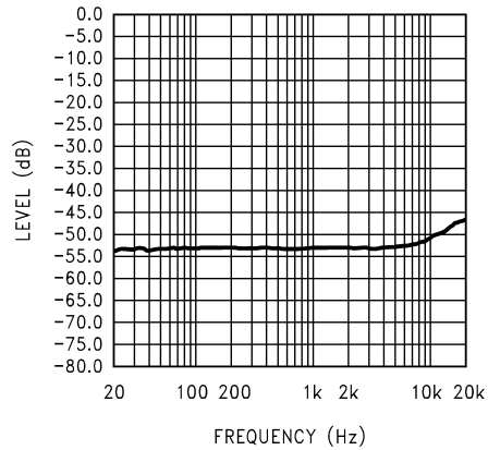
Input Floating
