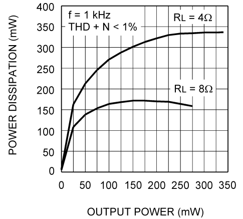
Power Dissipation vs Output Power, VDD = 2.6V
