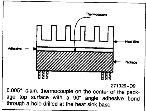
Figure 16-3. Case Temperature Measurement with Heat Sink
