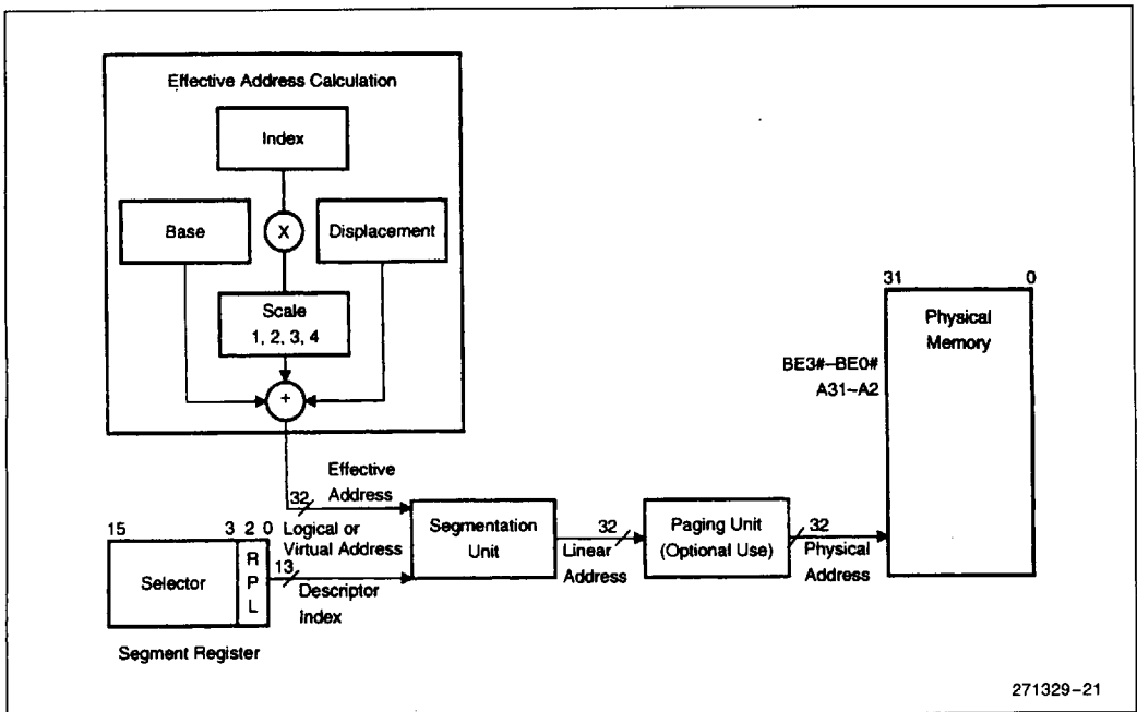
Figure 4-17. Address Translation
