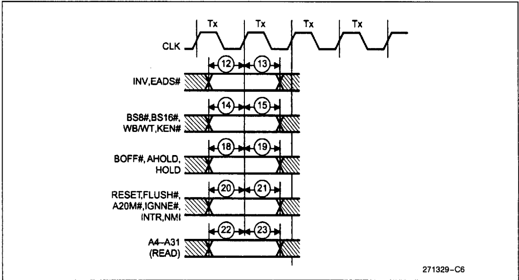
Figure 15-3. Input Setup and Hold Timing
