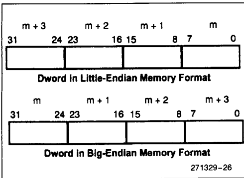
Figure 4-22. Big vs. Little Endian Memory Format
