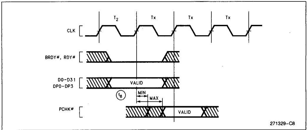
Figure 15-5. PCHK# Valid Delay Timing
