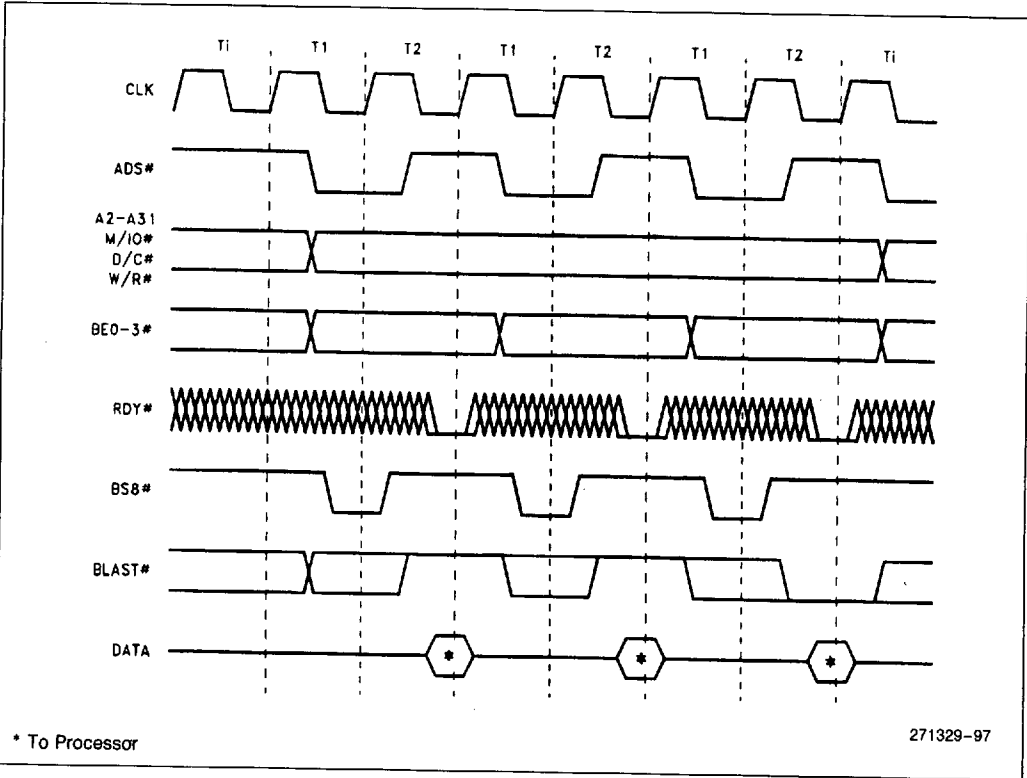
Figure 10-18. 8-Bit Bus Size Cycle
