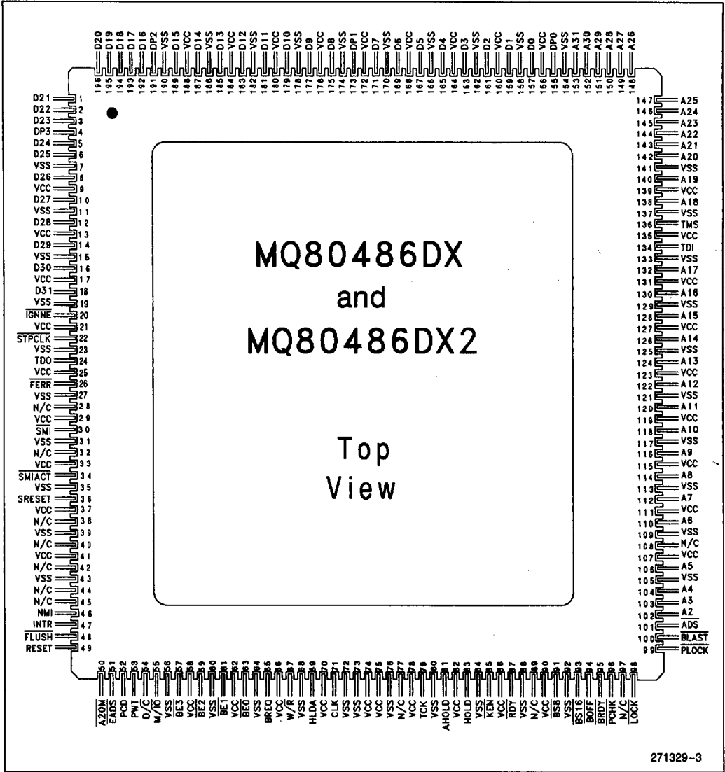
Figure 3-3. 196-Pin Ceramic Quad Flatpack (CQFP) Pin Configuration—View from Lid Side
