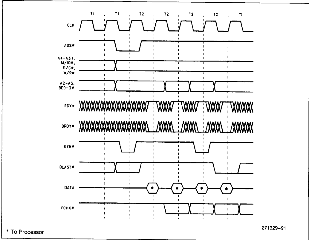
Figure 10-12. Burst Cacheable Cycle
