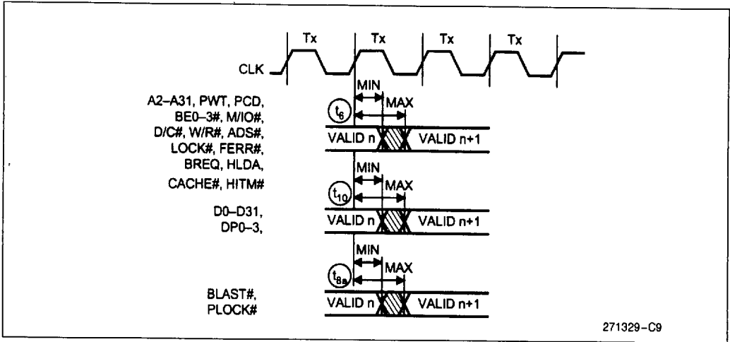
Figure 15-6. Output Valid Delay Timing
