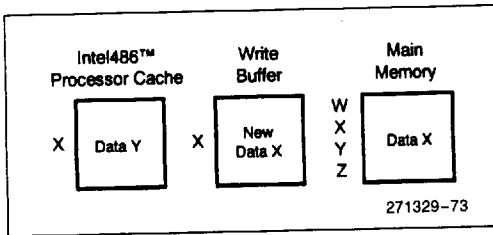
Figure 9-6. Reordering of a Reads with Write Buffers
