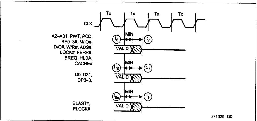
Figure 15-7. Maximum Float Delay Timing
