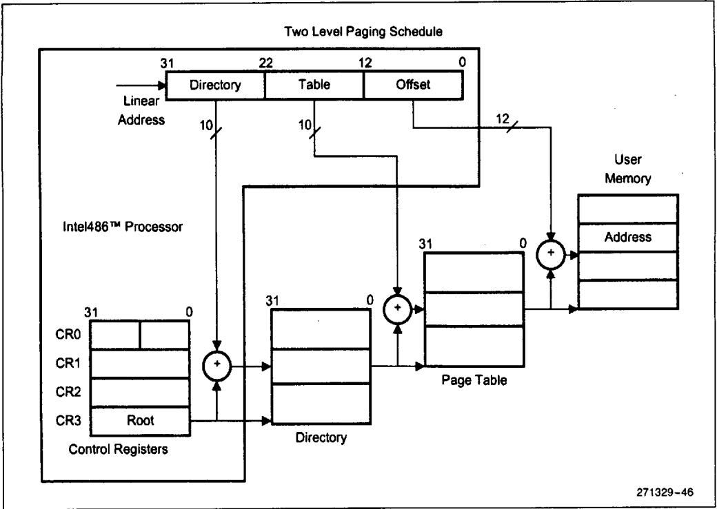
Figure 6-19. Paging Mechanism
