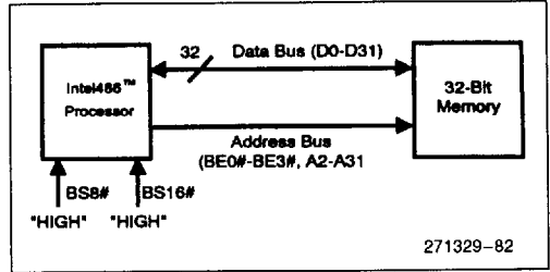
Figure 10-3. Military Intel486™ Processor with 32-Bit Memory
