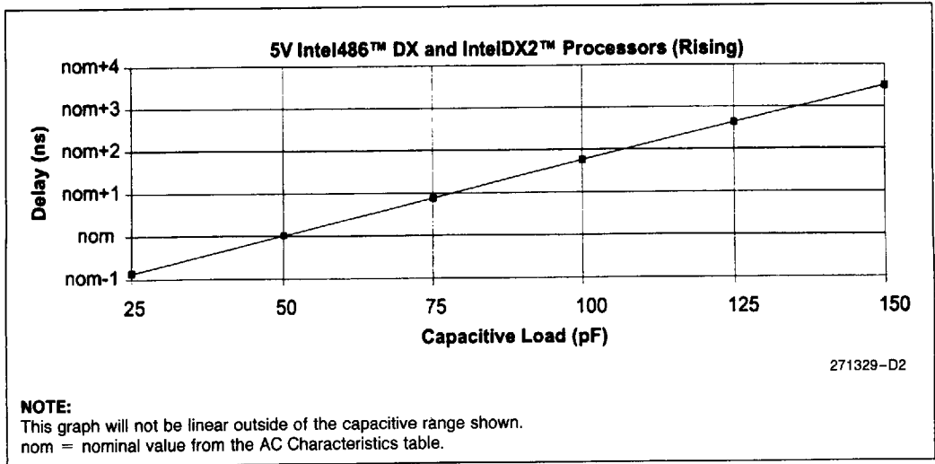
Figure 15-9. Typical Loading Delay versus Load Capacitance under Worst-Case Conditions for a Low-to-High Transition
