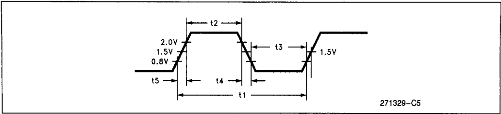
Figure 15-2. CLK Waveforms
