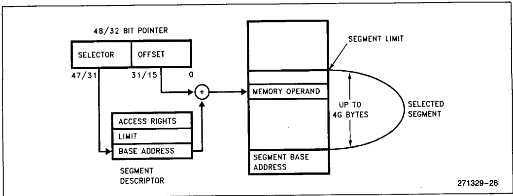
Figure 6-1. Protected Mode Addressing
