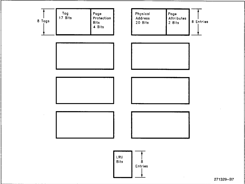
Figure 11-5. TLB Organization
