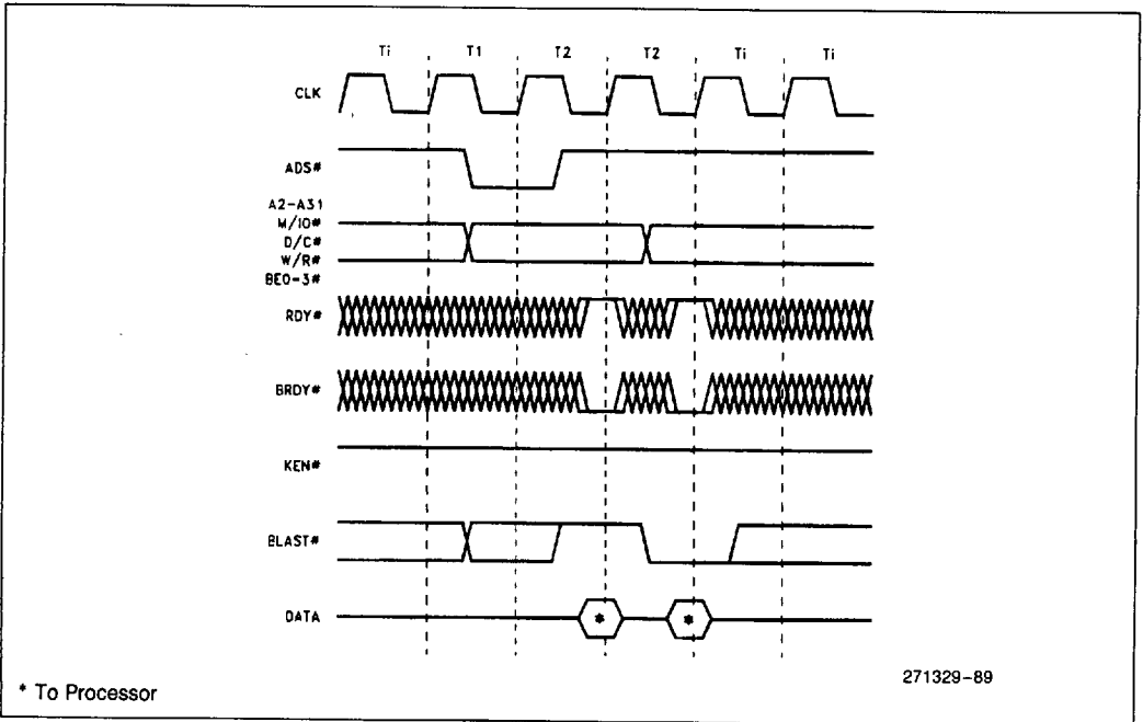
Figure 10-10. Non-Cacheable Burst Cycle
