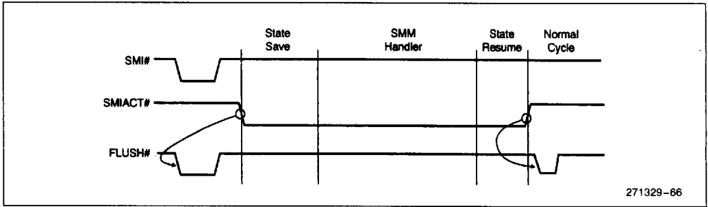
Figure 8-14. Cached SMM
