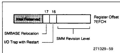
Figure 8-7. SMM Revision Identifier
