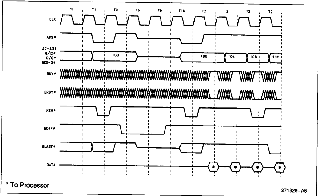
Figure 10-29. Restarted Read Cycle
