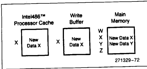
Figure 9-5. Reordering of a Reads with Write Buffers
