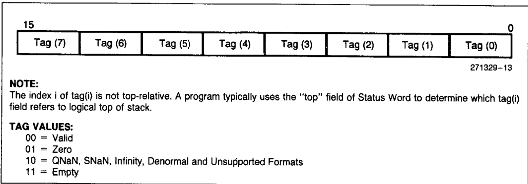
Figure 4-9. Floating Point Tag Word
