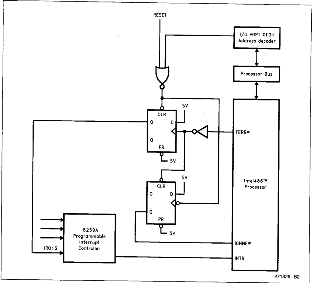
Figure 10-33. DOS-Compatible Numerics Error Circuit
