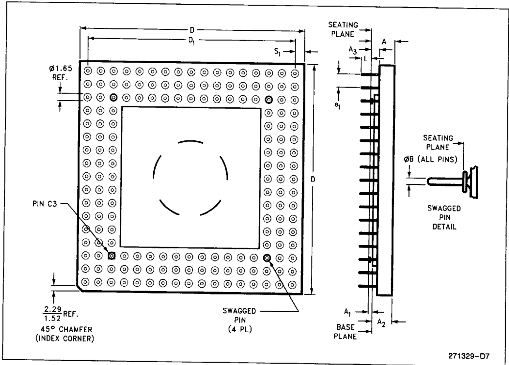
Figure 16-1. 168-Pin Ceramic PGA Package Dimensions
