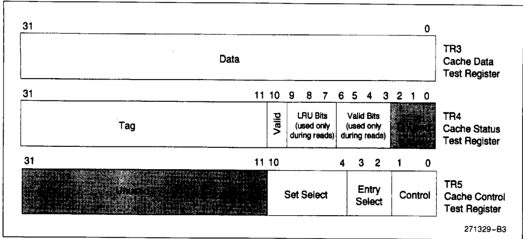
Figure 11-1. Cache Test Registers (All Military Intel486™ Processors Except the IntelDX4™ Processor)
