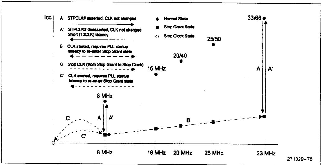
Figure 9-11. Supply Current Model for Stop Clock Modes and Transitions for the Military Intel486™ Processor
