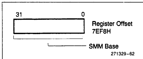
Figure 8-10. SMM Base Location
