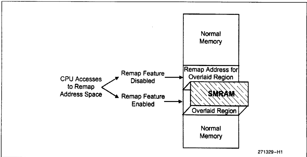
Figure D-2. Remapping Memory That Is Overlaid by SMRAM
