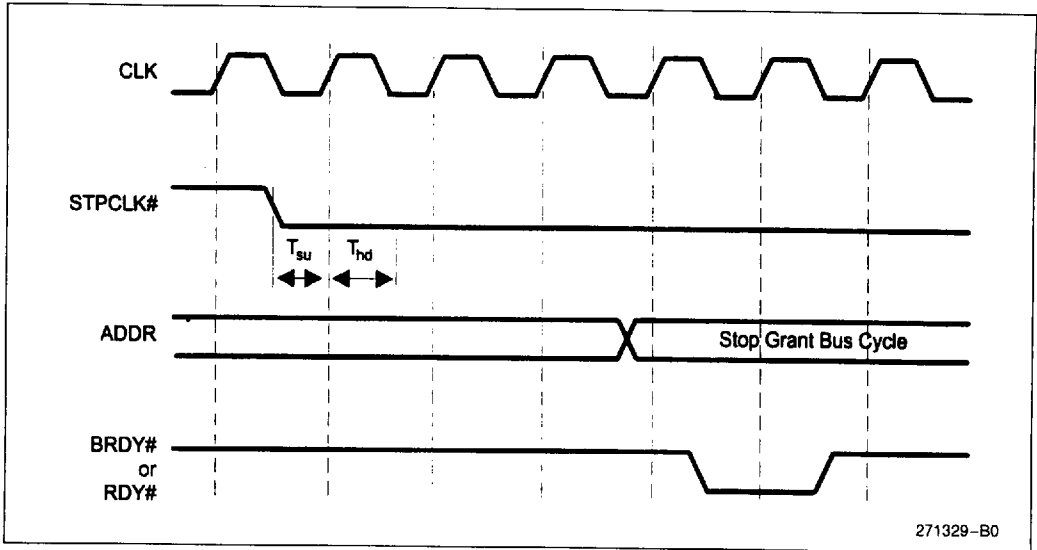
Figure 10-31. Stop Grant Bus Cycle
