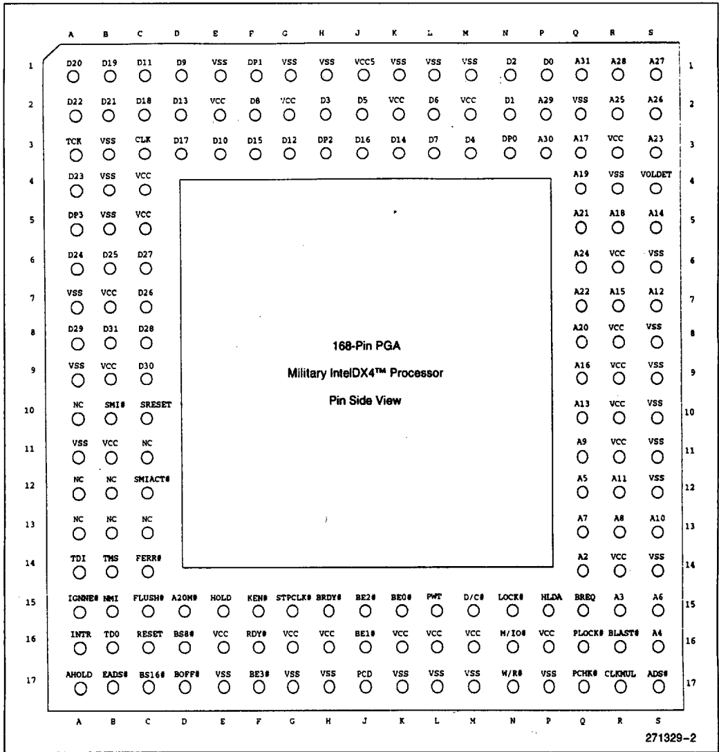
Figure 3-2. 168-Pin PGA Pinout Diagram (Pin Side) for the Military IntelDX4™ Processor
