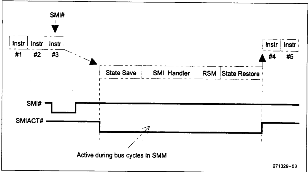
Figure 8-1. Basic SMI # Interrupt Service
