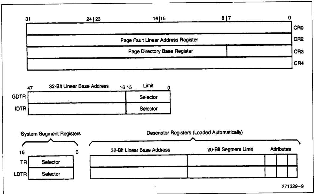
Figure 4-5. System Level Registers
