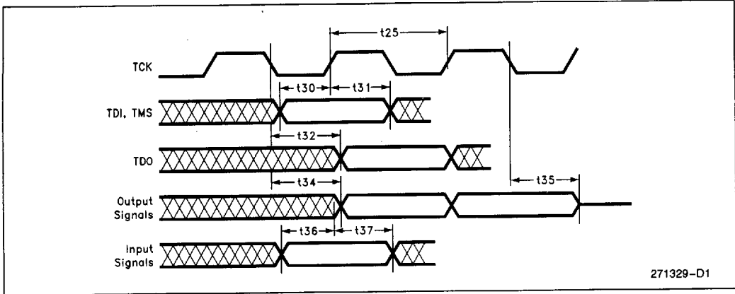
Figure 15-8. Test Signal Timing Diagram
