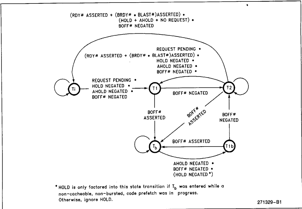
Figure 10-32. Bus State Diagram
