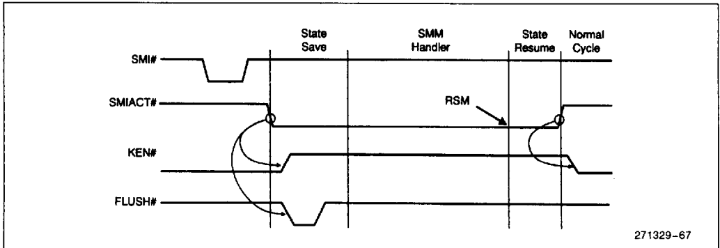
Figure 8-15. Non-Cached SMM
