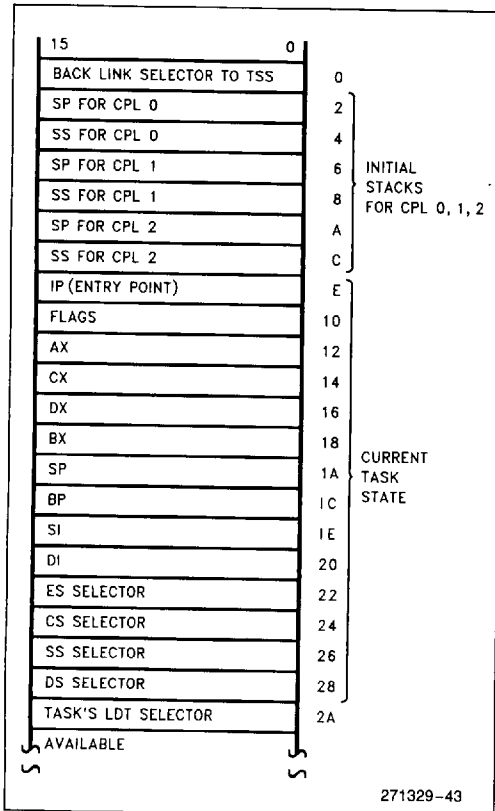
Figure 6-16. 80286 TSS
