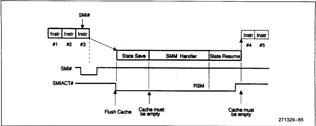
Figure 8-13. FLUSH# Mechanism during SMM
