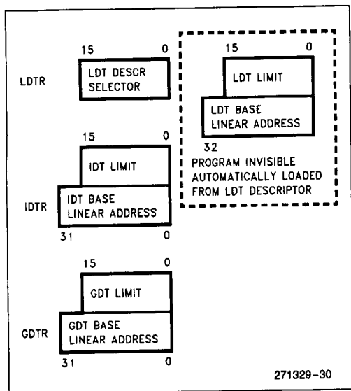
Figure 6-3. Descriptor Table Registers
