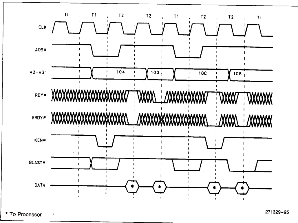
Figure 10-16. Interrupted Burst Cycle
