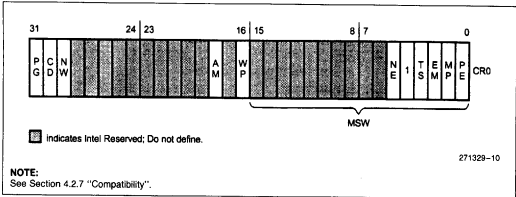
Figure 4-6. Control Register 0
