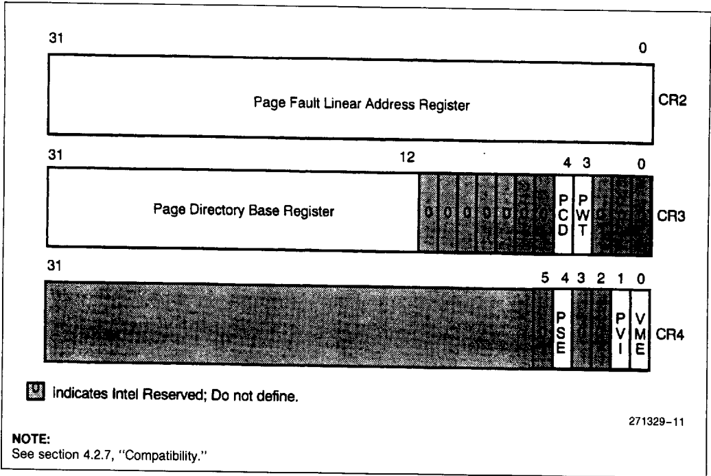
Figure 4-7. Control Registers 2, 3 and 4
