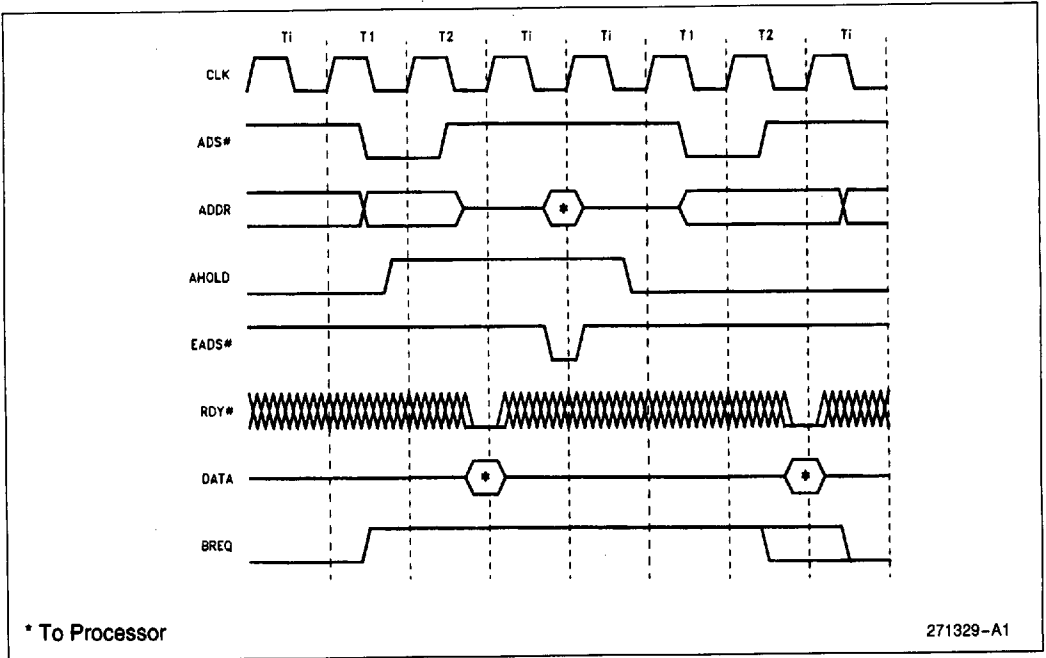
Figure 10-22. Fast Internal Cache Invalidation Cycle
