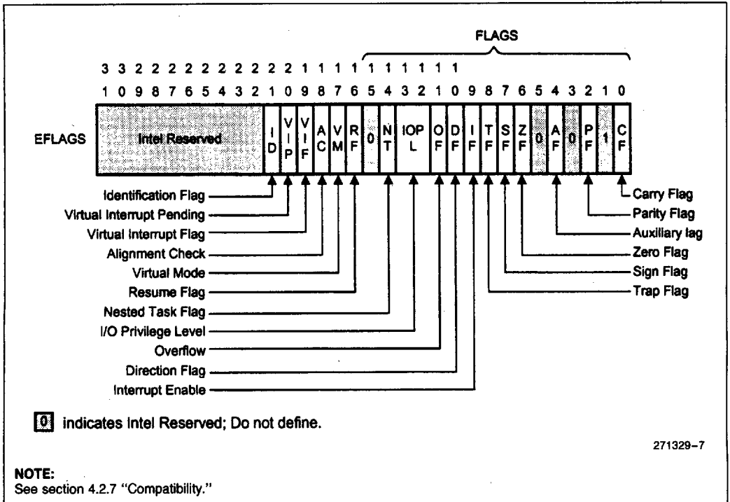
Figure 4-3. Flag Registers
