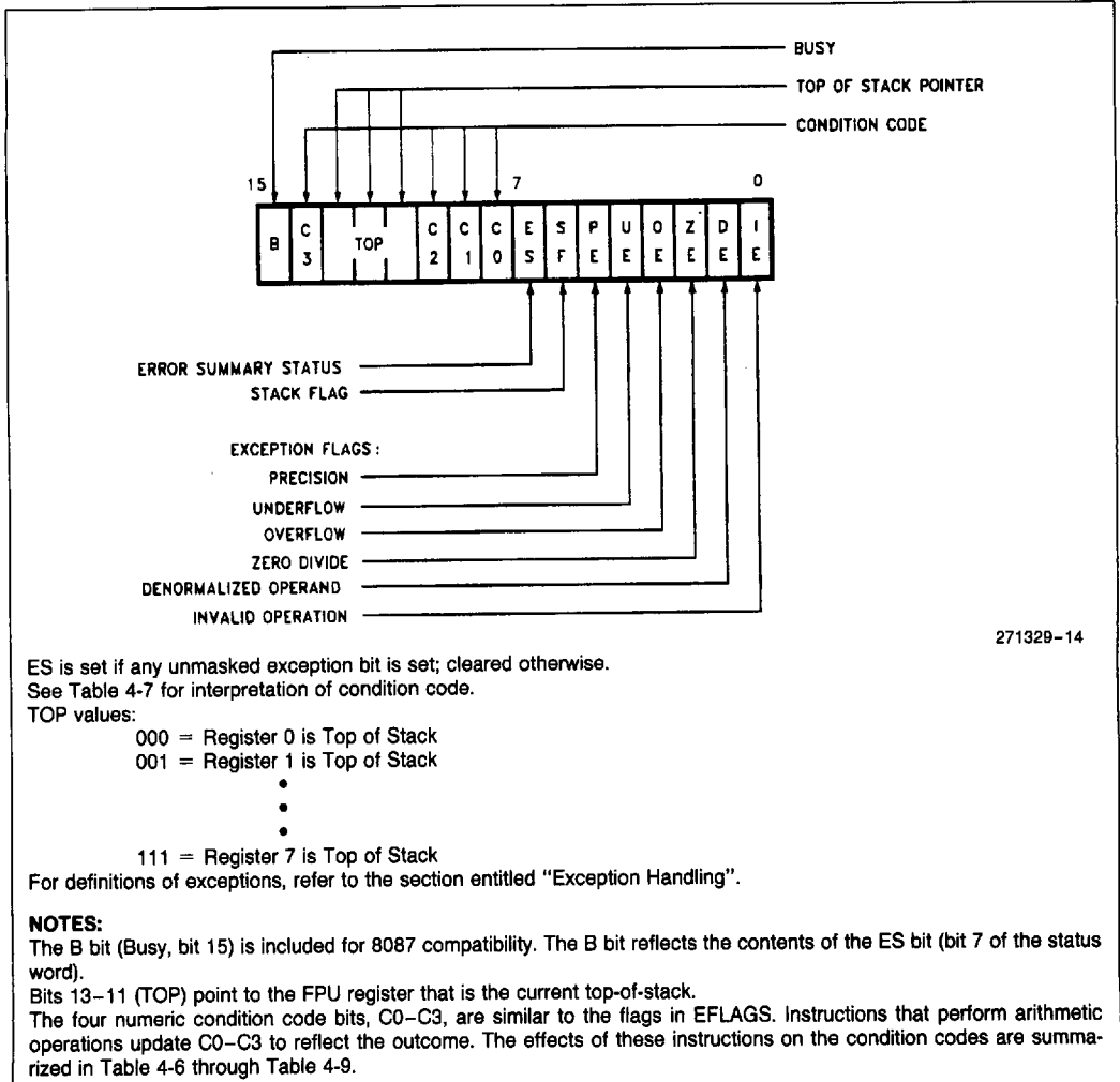
Figure 4-10. Floating Point Status Word
