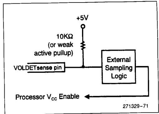
Figure 9-4. Voltage Detect (VOLDET) Sense Pin
