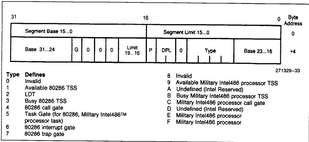
Figure 6-6. System Segment Descriptors
