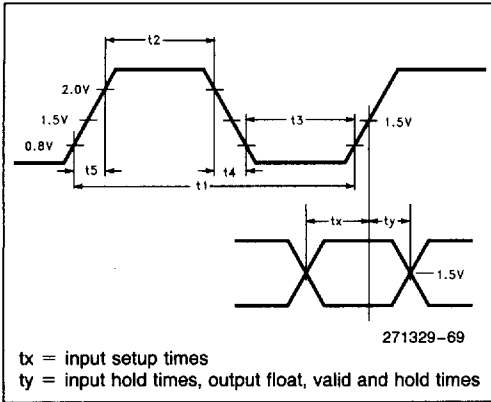
Figure 9-2. CLK Waveform
