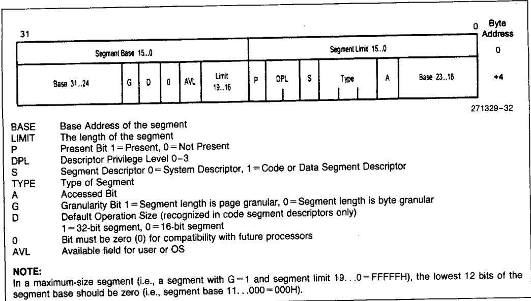
Figure 6-5. Segment Descriptors
