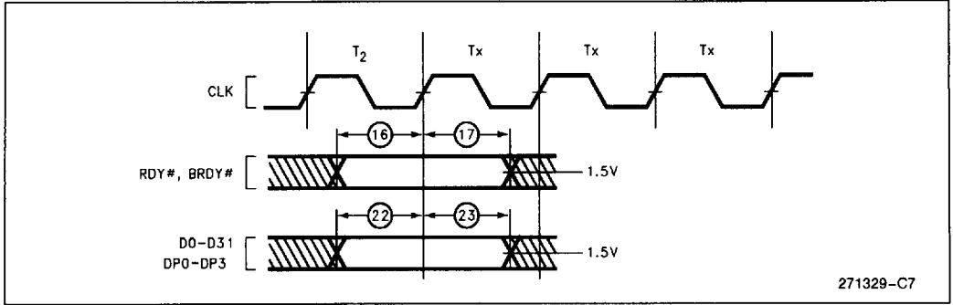
Figure 15-4. Input Setup and Hold Timing
