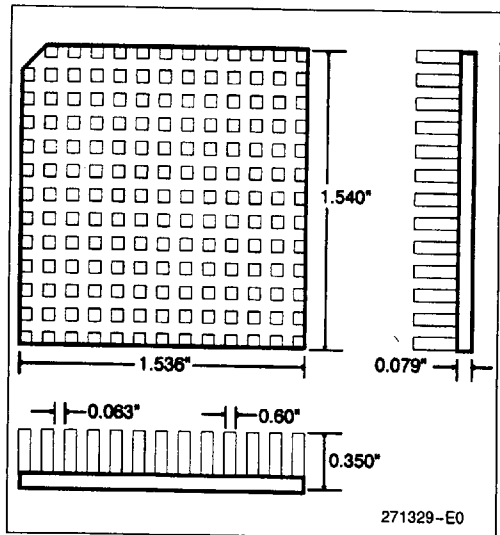
Figure 16-4. Sample IntelDX4™ Processor PGA Heat Sink
