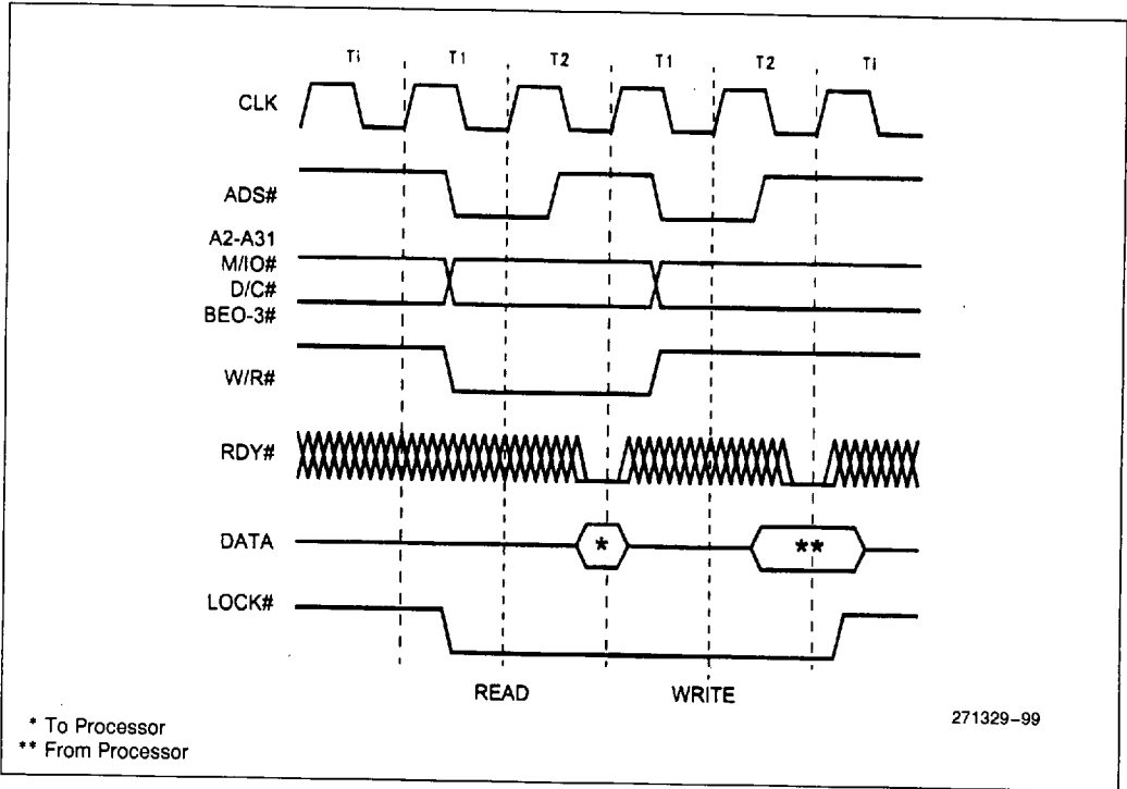
Figure 10-20. Locked Bus Cycle
