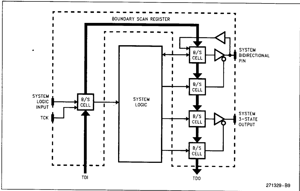
Figure 11-7. Logical Structure of Boundary Scan Register
