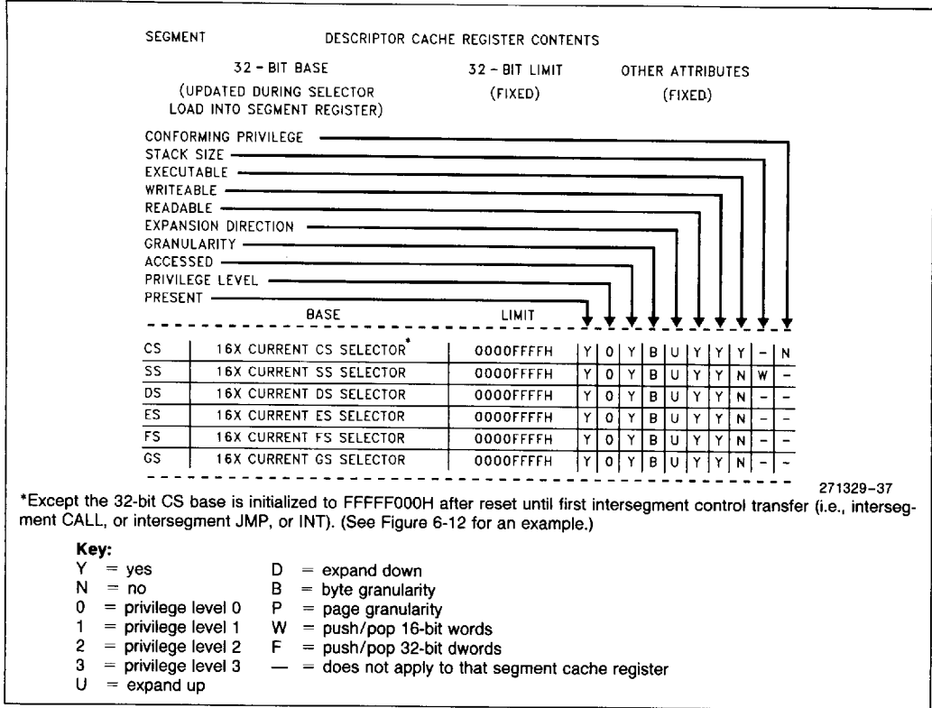
Figure 6-10. Segment Descriptor Caches for Real Address Mode (Segment Limit and Attributes Are Fixed)
