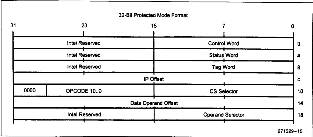
Figure 4-11. Protected Mode FPU Instructions and Data Pointer Image in Memory, 32-Bit Format
