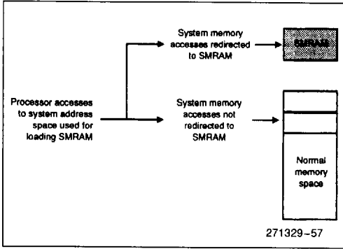
Figure 8-5. Redirecting System Memory Addresses to SMRAM
