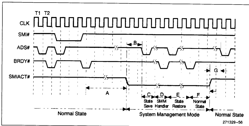
Figure 8-4. Military Intel486™ Processor SMIACK# Timing
