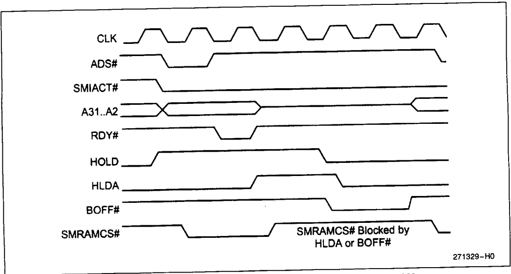
Figure D-1. Blocking Other Bus Masters from Accessing SMRAM
