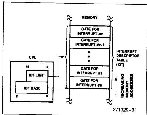
Figure 6-4. Interrupt Descriptor Table Register Use
