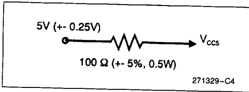
Figure 15-1. IntelDX4™ Processor V_{CC5} Current Limiting Resistor
