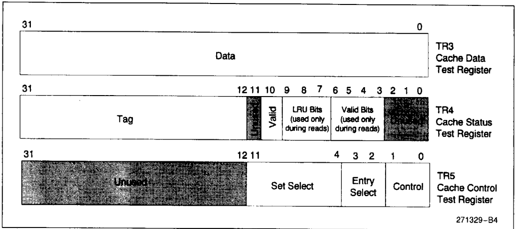
Figure 11-2. IntelDX4™ Processor Cache Test Registers
