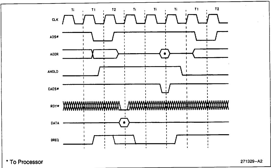
Figure 10-23. Typical Internal Cache Invalidation Cycle
