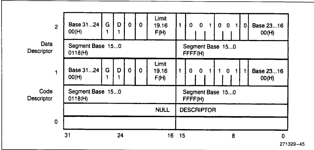
Figure 6-18. GDT Descriptors for Simple System
