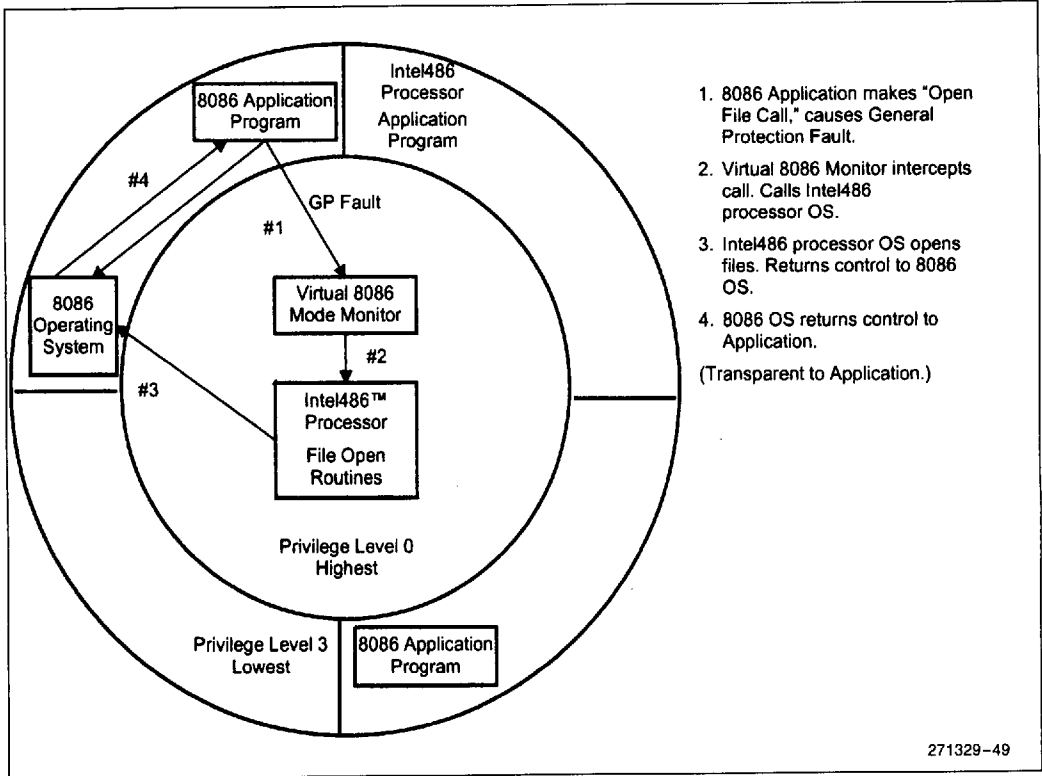
Figure 6-25. Virtual 8086 Environment Interrupt and Call Handling
