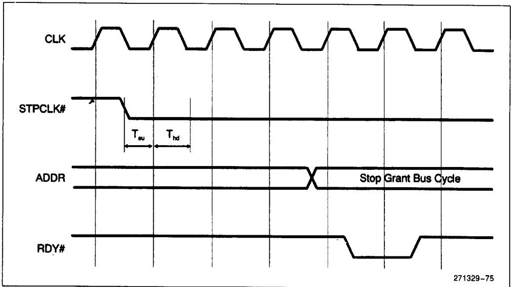
Figure 9-8. Stop Clock Protocol
