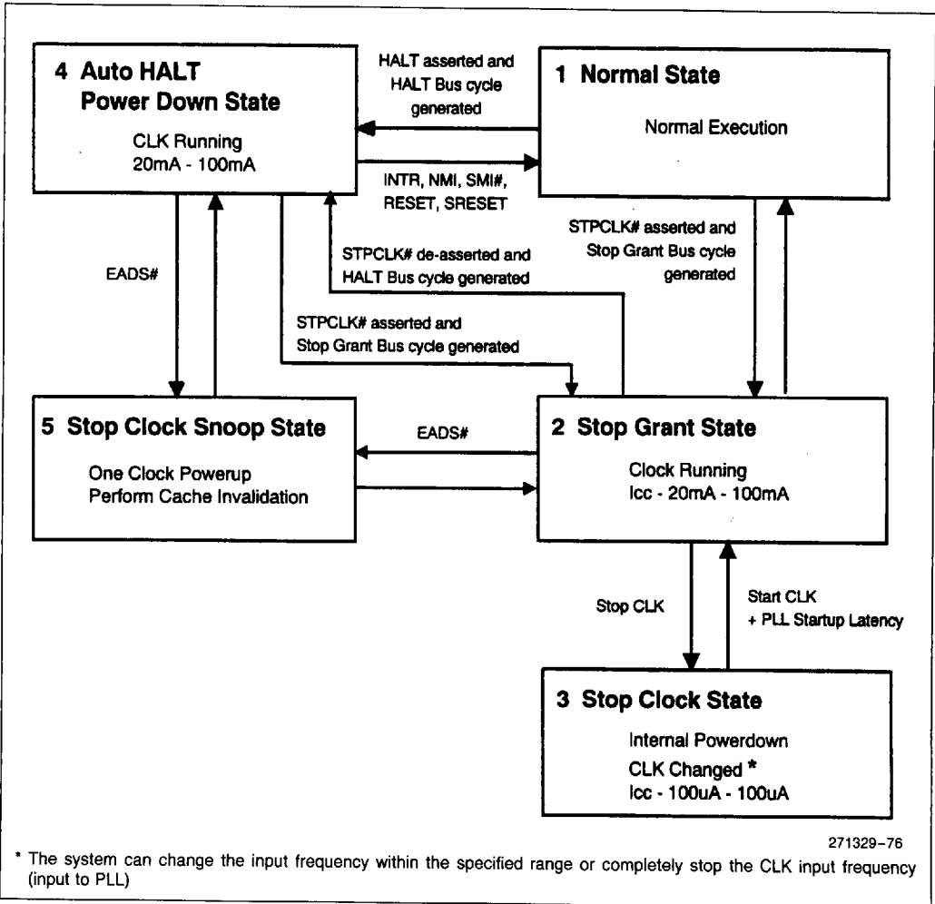
Figure 9-9. Military Intel486™ Processor Family Stop Clock State Machine
