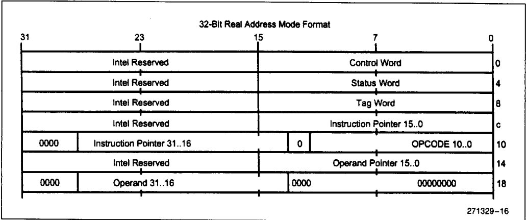
Figure 4-12. Real Mode FPU Instruction and Data Pointer Image in Memory, 32-Bit Format
