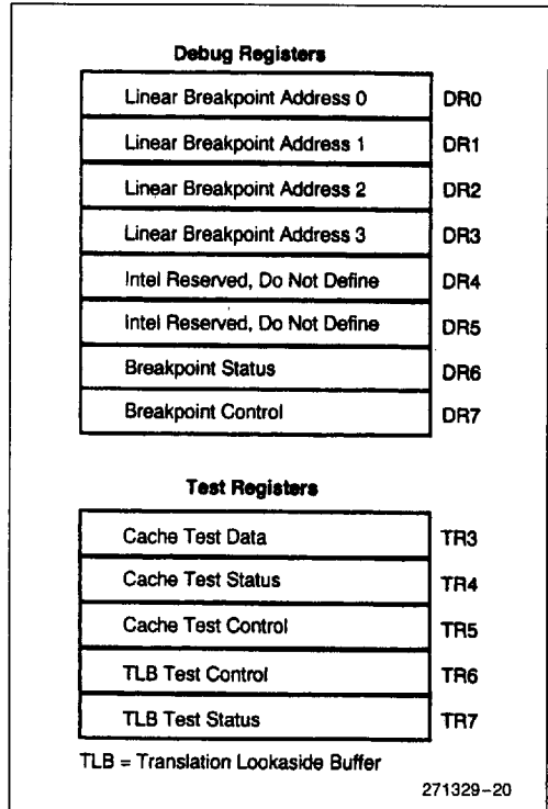
Figure 4-16. Debug and Test Registers
