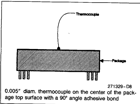
Figure 16-2. Case Temperature Measurement without Heat Sink
