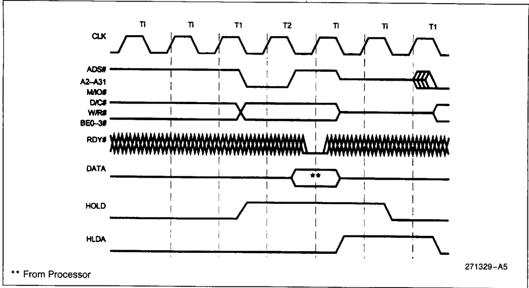
Figure 10-26. HOLD/HLDA Cycles
