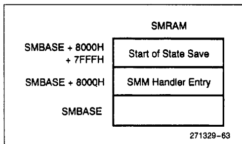
Figure 8-11. SMRAM Usage
