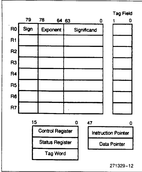
Figure 4-8. Floating Point Registers
