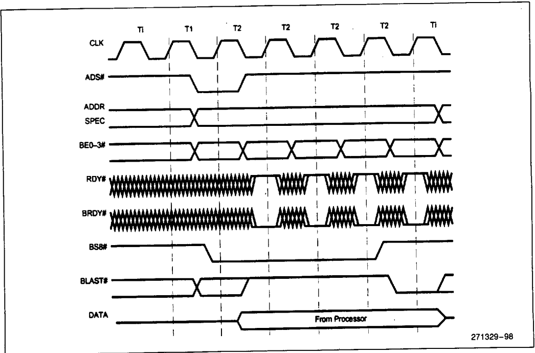
Figure 10-19. Burst Write as a Result of BS8# or BS16#
