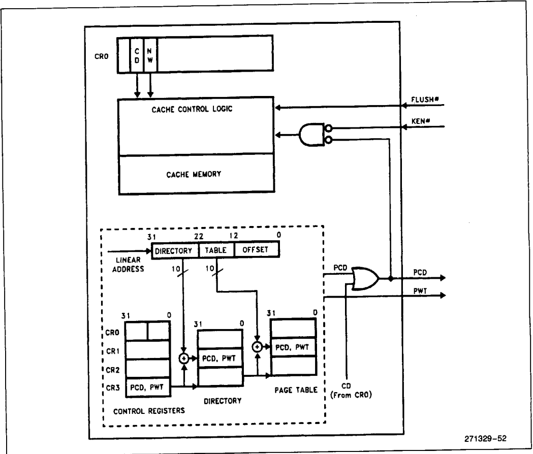
Figure 7-3. Page Cacheability
