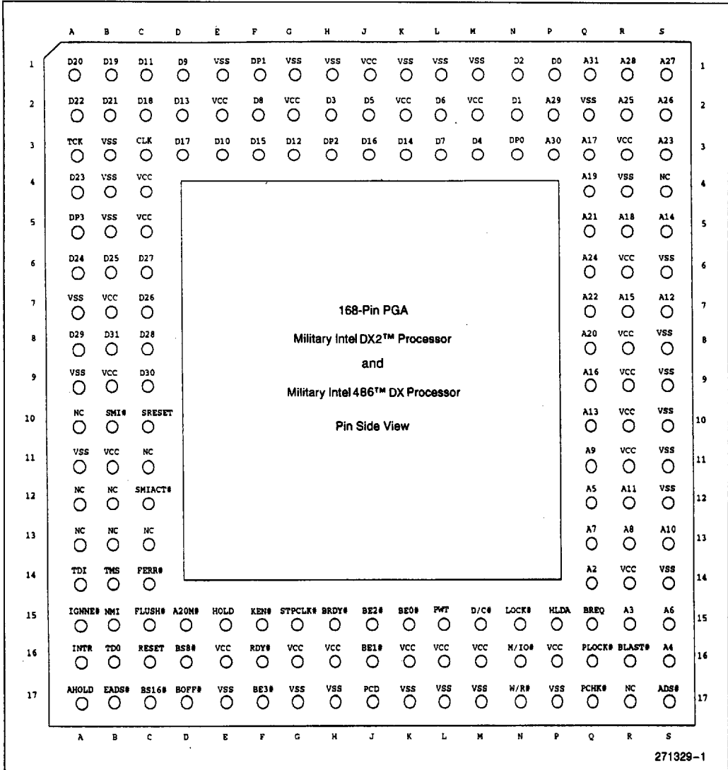
Figure 3-1. Package Diagram for 168-Pin PGA Package of the Military IntelDX2™ Processor and the Military Intel486™ DX Processor
