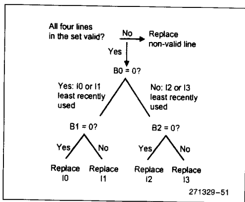
Figure 7-2. On-Chip Cache Replacement Strategy
