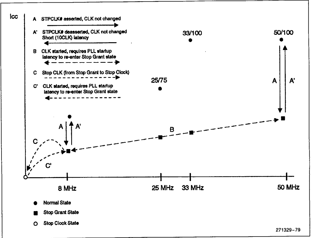
Figure 9-12. Supply Current Model for Stop Clock Modes and Transitions for the IntelDX4™ Processor
