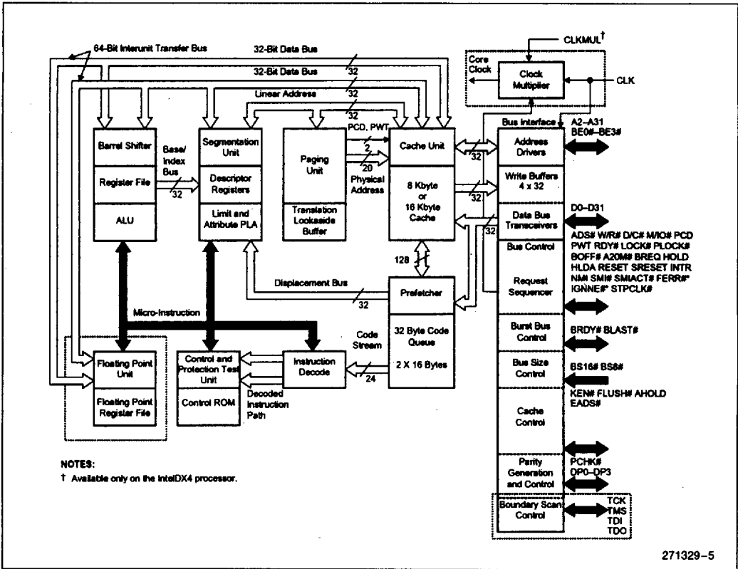
Figure 4-1. Military Intel486™ Processor Block Diagram
