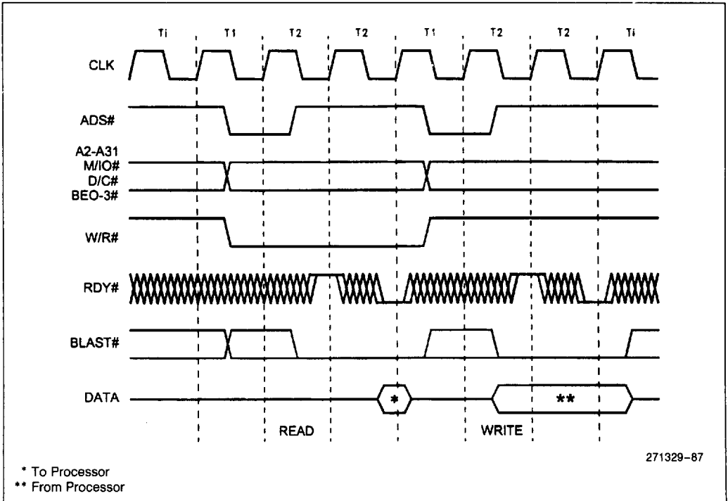
Figure 10-8. Basic 3-3 Bus Cycle
