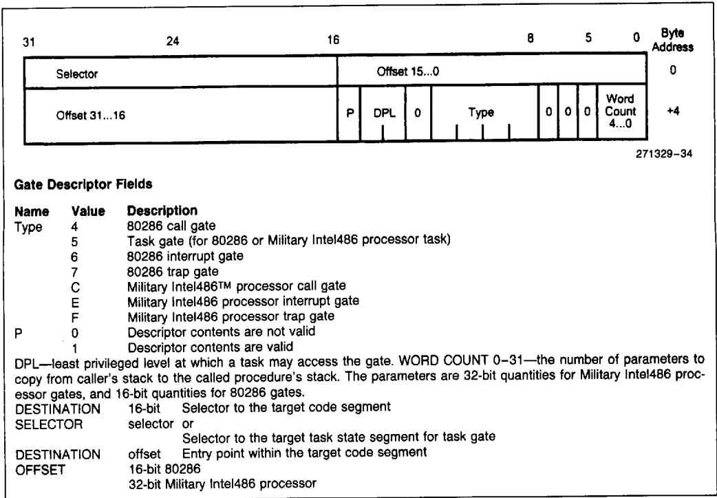
Figure 6-7. Gate Descriptor Formats
