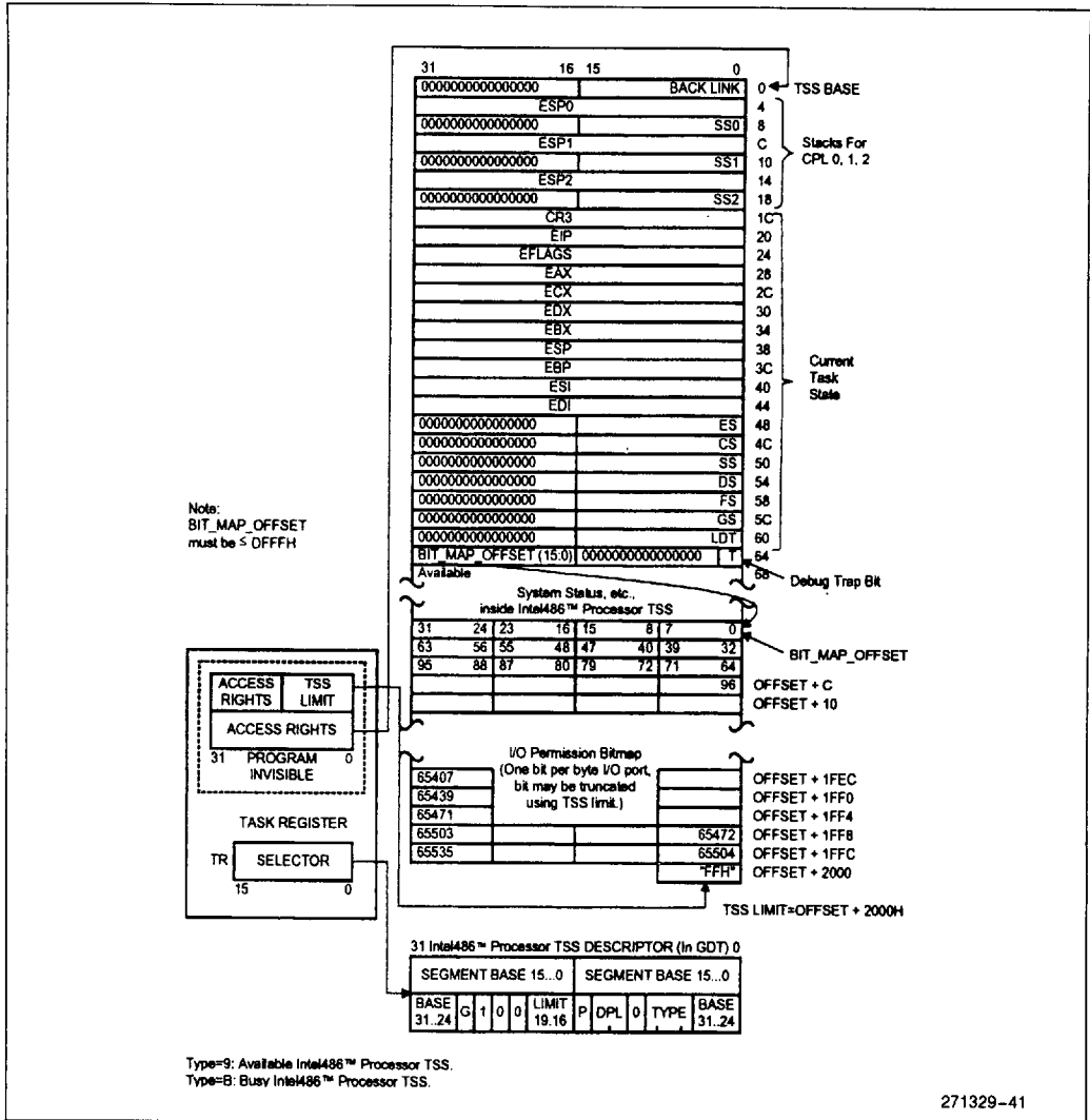
Figure 6-14. Military Intel486™ Processor TSS and TSS Registers
