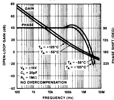
OPEN-LOOP GAIN, PHASE vs FREQUENCY ( C_{OC} = 0pF )
