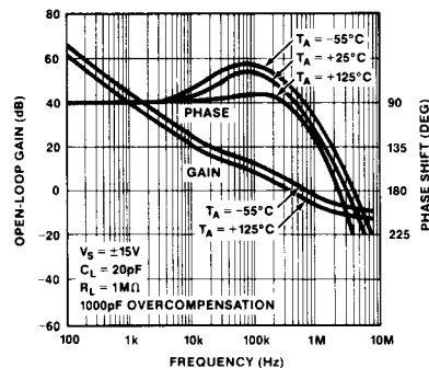
OPEN-LOOP GAIN, PHASE vs FREQUENCY ( C_{OC} = 1000pF )
