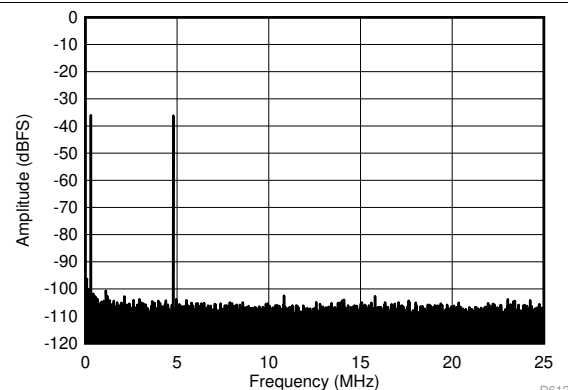
f_{IN1} = 46\text{ MHz} , f_{IN2} = 50\text{ MHz} , IMD3 = 103 dBFS, each tone at -36 dBFS
