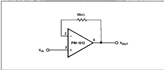
FIGURE 5: Unity-Gain Follower
