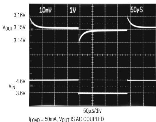
LINE TRANSIENT
