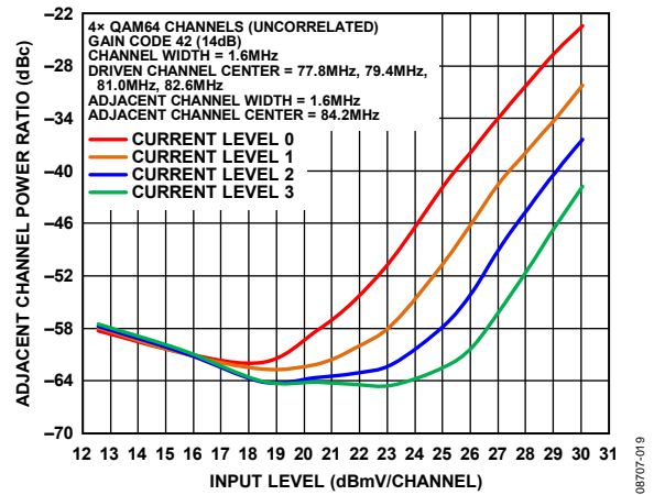
Figure 20. ACPR vs. Input Level for 4x QAM64 Channels
