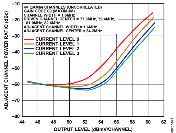
Figure 21. ACPR vs. Output Level for 4x QAM64 Channels
