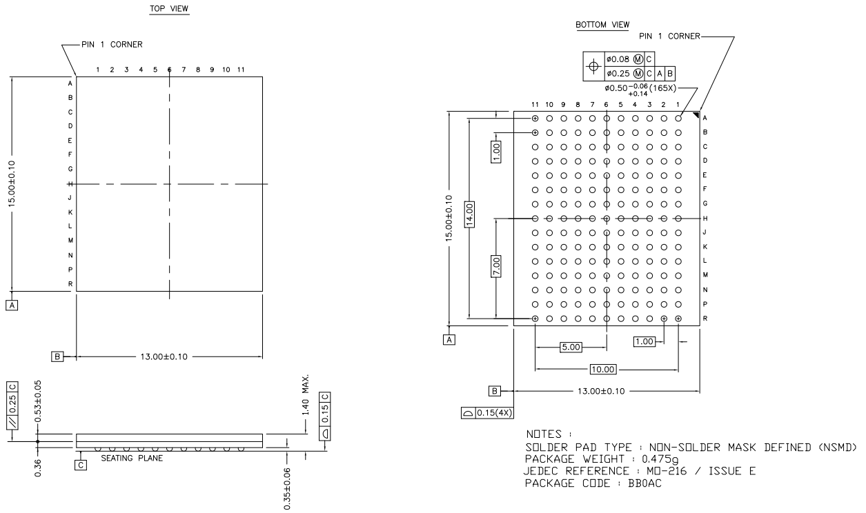
Figure 3. 165-ball FBGA (13 × 15 × 1.4 mm), 51-85180
