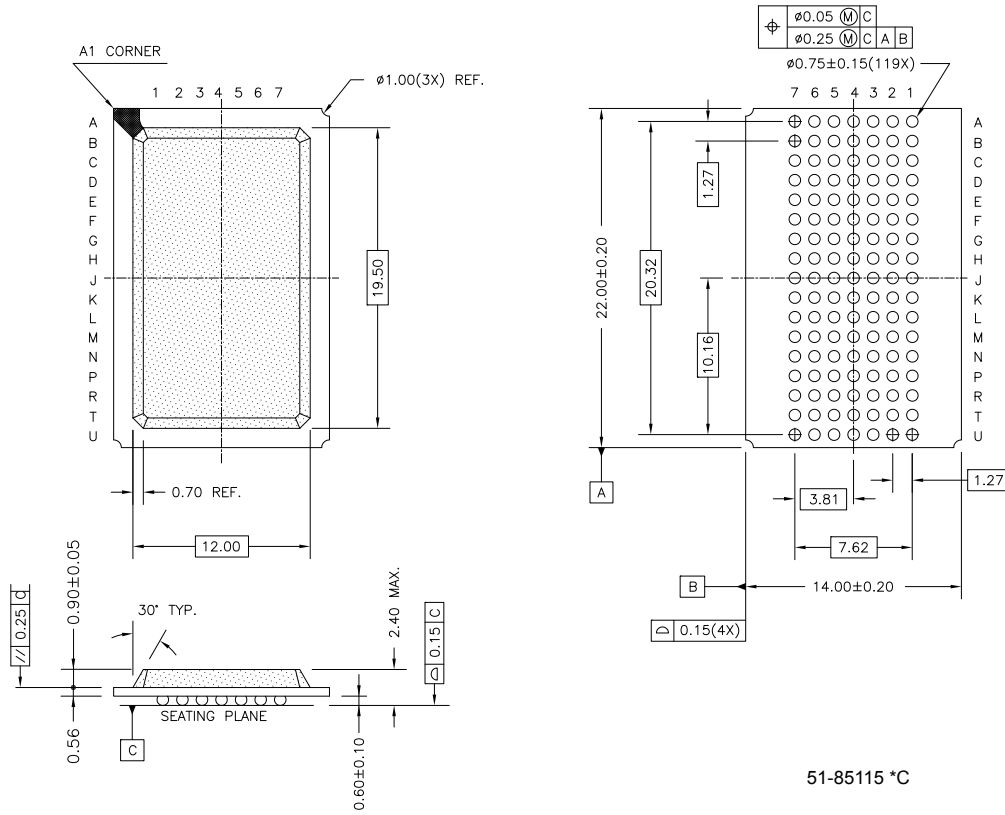
Figure 2. 119-ball BGA (14 × 22 × 2.4 mm), 51-85115
